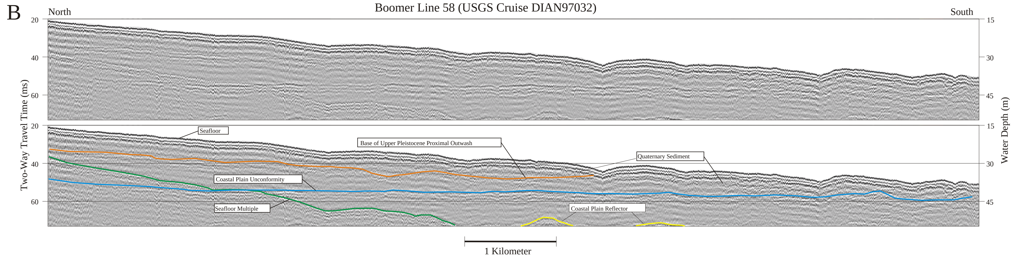
Figure 5b. Processed boomer subbottom profile with interpretation of reflection horizons. This profile is located in the eastern part of the study area. Water depth in meters is assuming a seismic velocity of 1500 m/s. See figures 4 and 6 for profile location.
