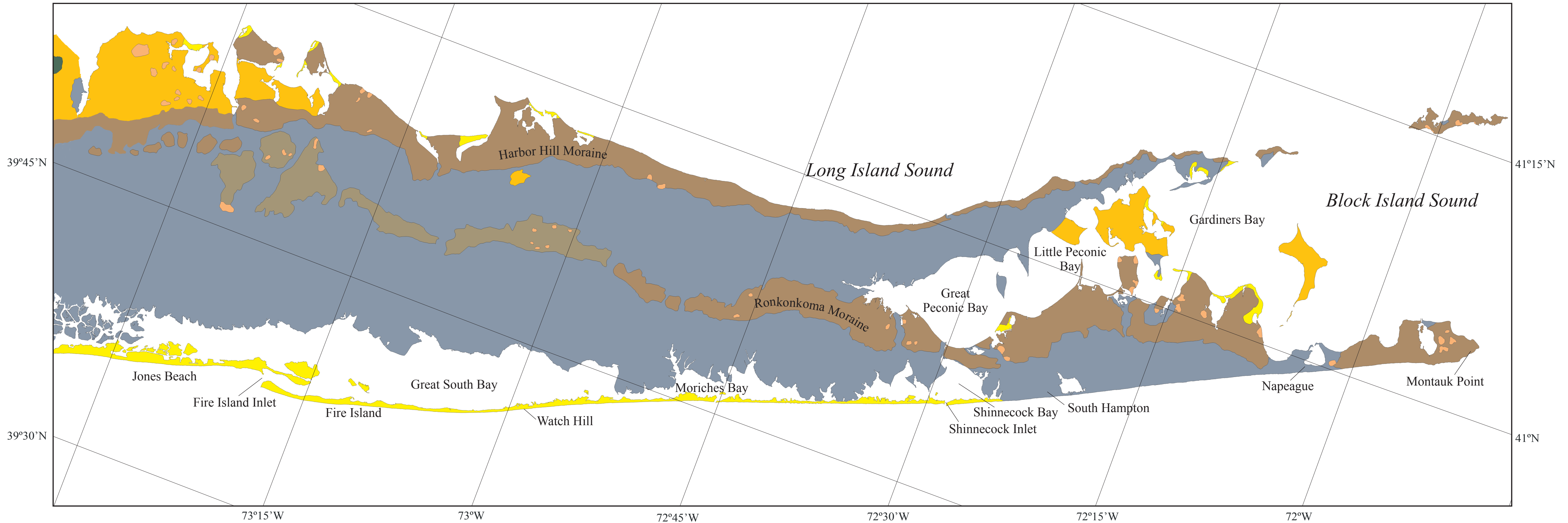
Figure 2. Surficial geologic map of Long Island, New York (modified from New York State Geological Survey, 1986; http://www.nysm.nysed.gov/gis.html ).
