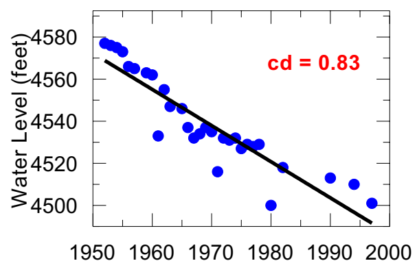
F. Annual water levels ( WL_{LC} ) in Little Chino Valley
