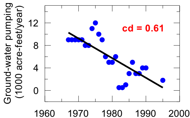
A. Annual pumping for irrigation (GWP) in Big Chino Valley
