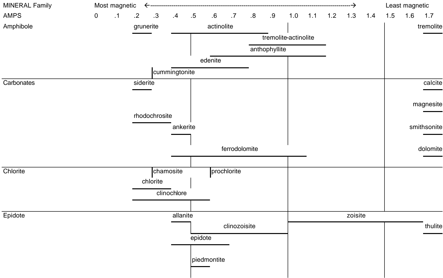
Figure 2 Magnetic Susceptibilities of Minerals by Families
