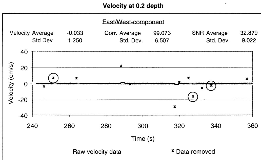
Figure 5. Example plot of raw and filtered data, collected near the wetlands adjacent to canal C-111, with removal of additional extreme outliers. (Average and standard deviation values were calculated from raw velocity data (*) as was the 21-point running average (—). Data removed by the filters are circled and remaining outliers are identified by an asterisk (*).)
