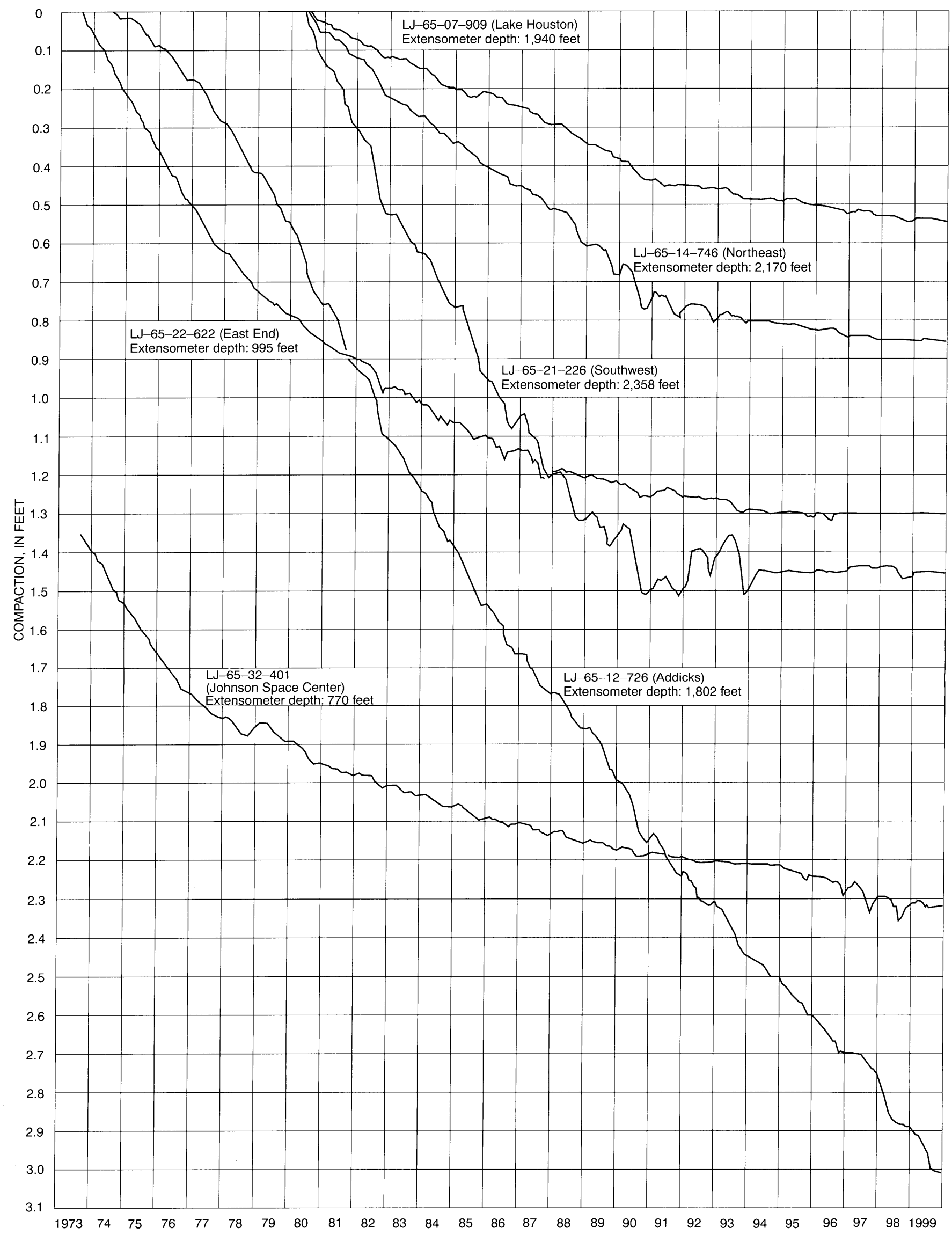
Figure 8. Graphs showing measured compaction of subsurface material, 1973-99, at extensometer sites shown in figure 7.
