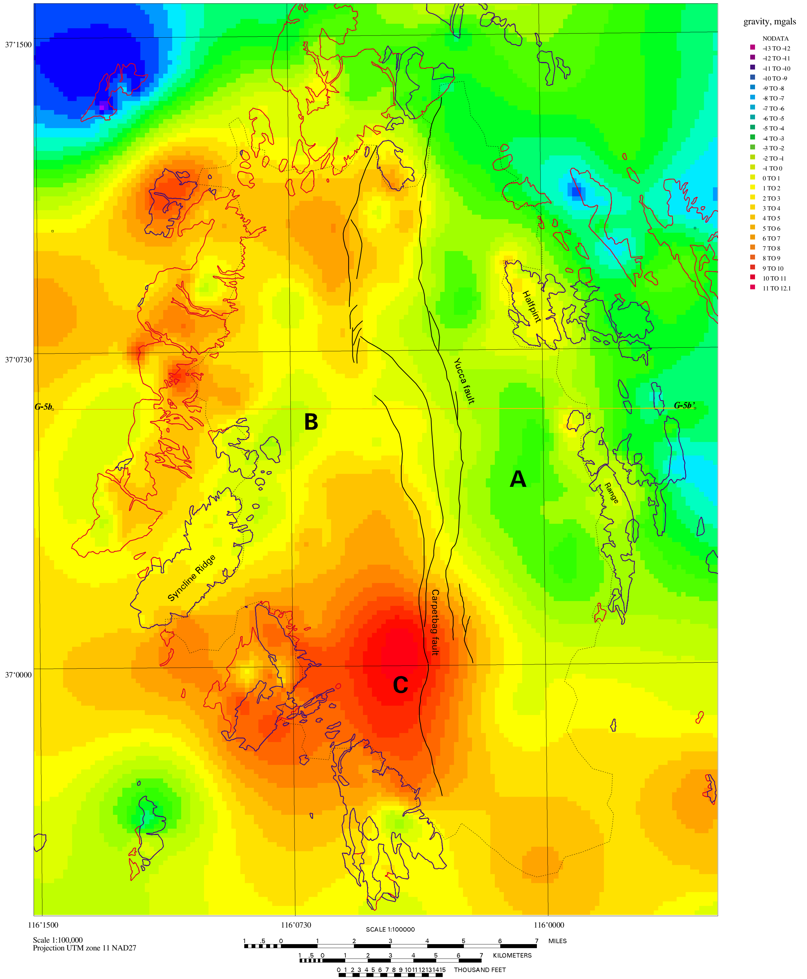
figure 1. Basement gravity beneath Yucca Flat red outlines, non-carbonate pre-Tertiary basement rocks; blue outlines, Paleozoic carbonate rocks; orange line, G-5b cross-section line; black lines, faults; anomalies A, B, and C shown by corresponding letters on the map; dashed outline, Yucca Flat basin study area
