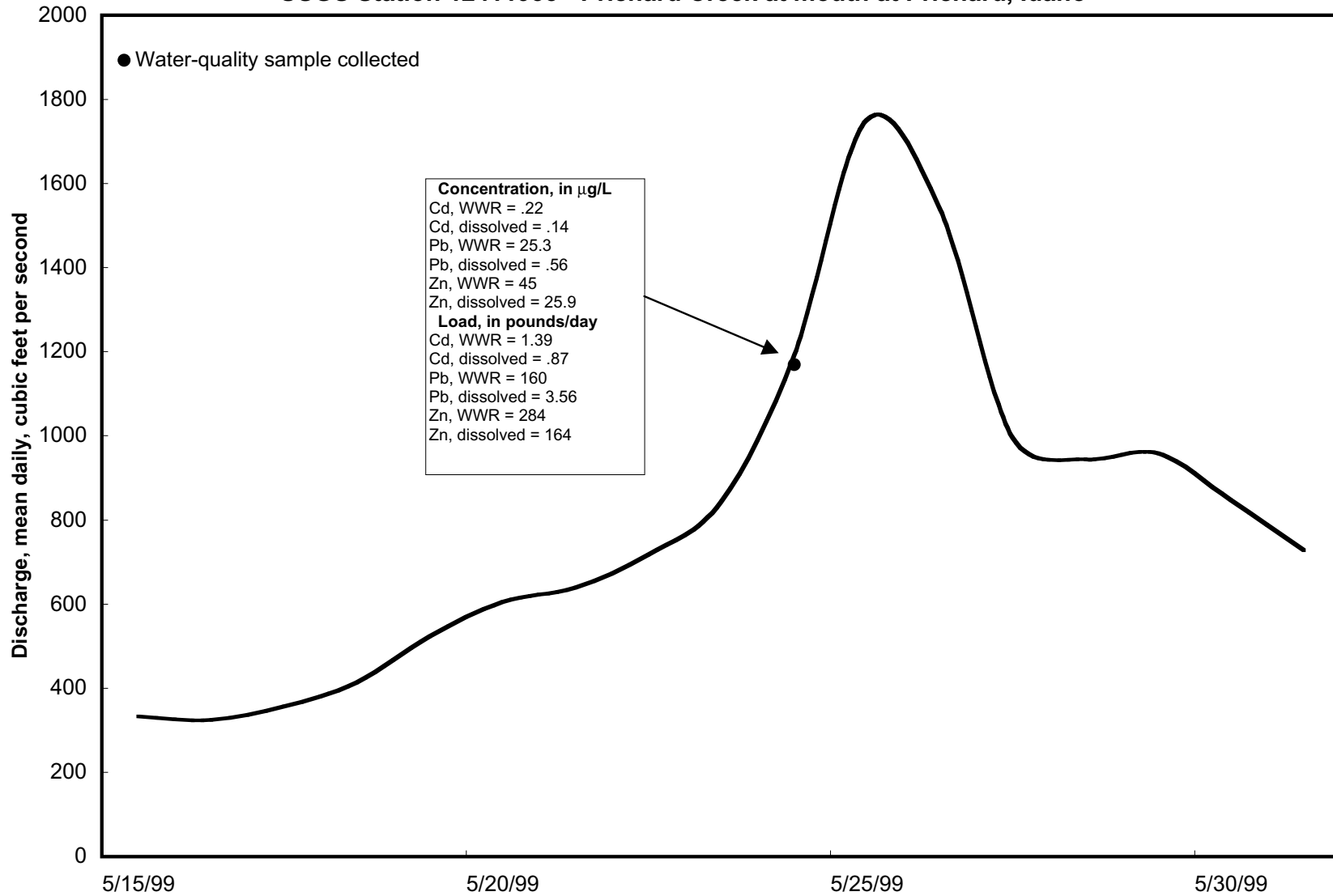
Figure 11. Near-peak portion of 1999 snowmelt-runoff hydrograph with concentrations and loads of cadmium, lead, and zinc at Prichard Creek at mouth at Prichard, Idaho. (USGS, U.S. Geological Survey; \mu\text{g/L} , micrograms per liter; WWR, whole-water recoverable)
