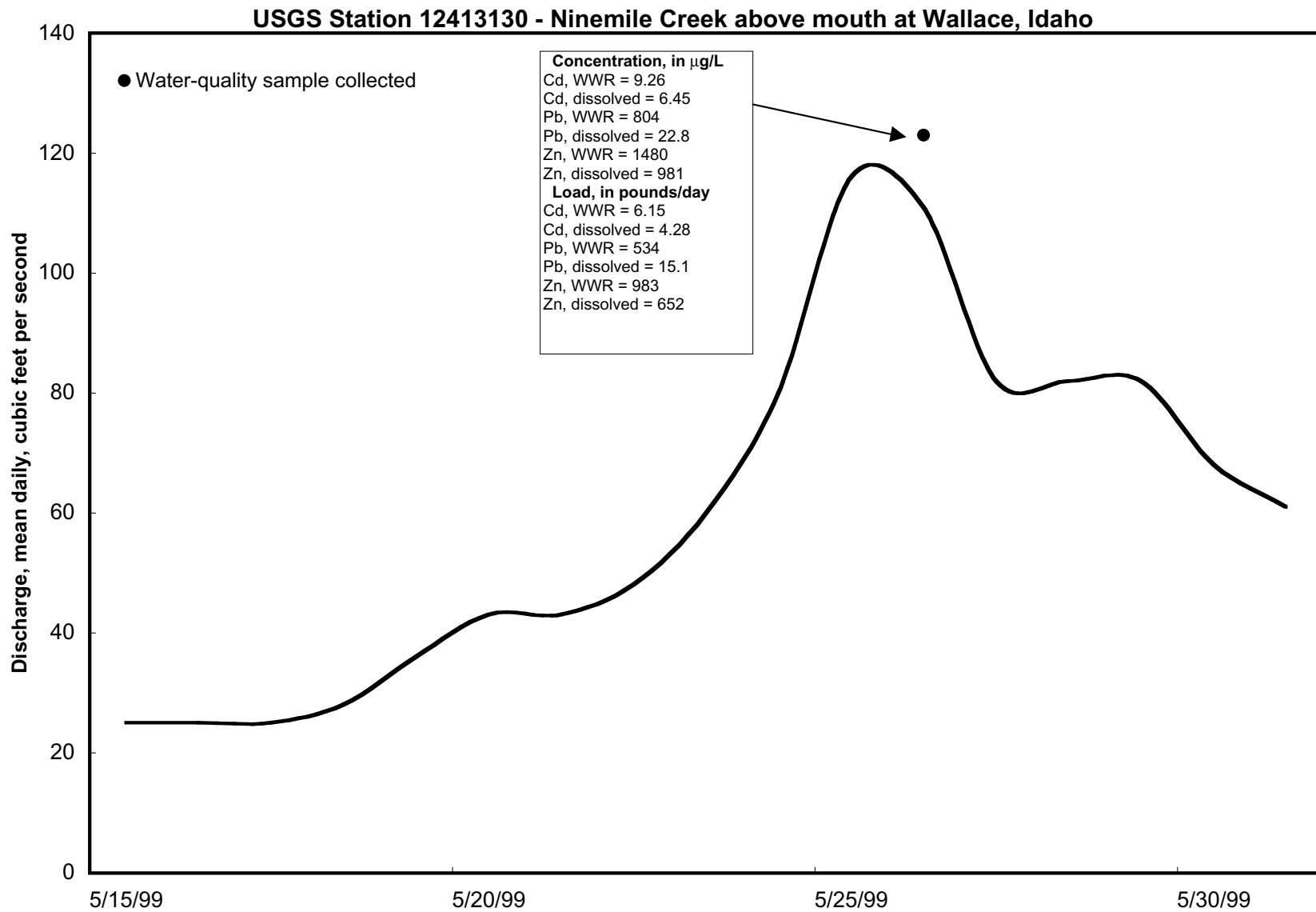
Figure 7. Near-peak portion of 1999 snowmelt-runoff hydrograph with concentrations and loads of cadmium, lead, and zinc at Ninemile Creek above mouth at Wallace, Idaho. (USGS, U.S. Geological Survey; \mu\text{g/L} , micrograms per liter; WWR, whole-water recoverable)
