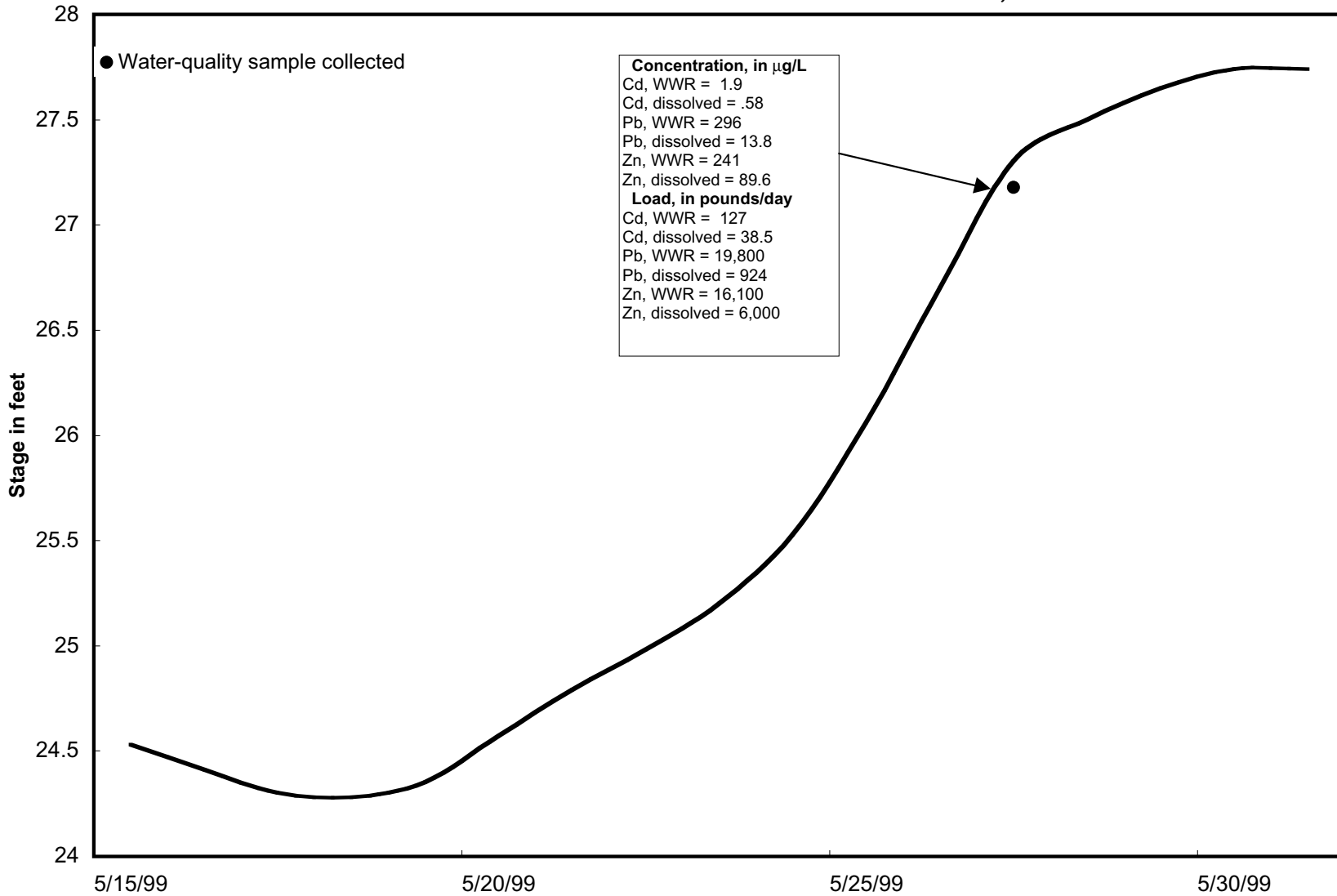
Figure 15. Near-peak portion of 1999 snowmelt-runoff hydrograph with concentrations and loads of cadmium, lead, and zinc at Coeur d'Alene River near Harrison, Idaho. (USGS, U.S. Geological Survey; \mu\text{g/L} , micrograms per liter; WWR, whole-water recoverable)
