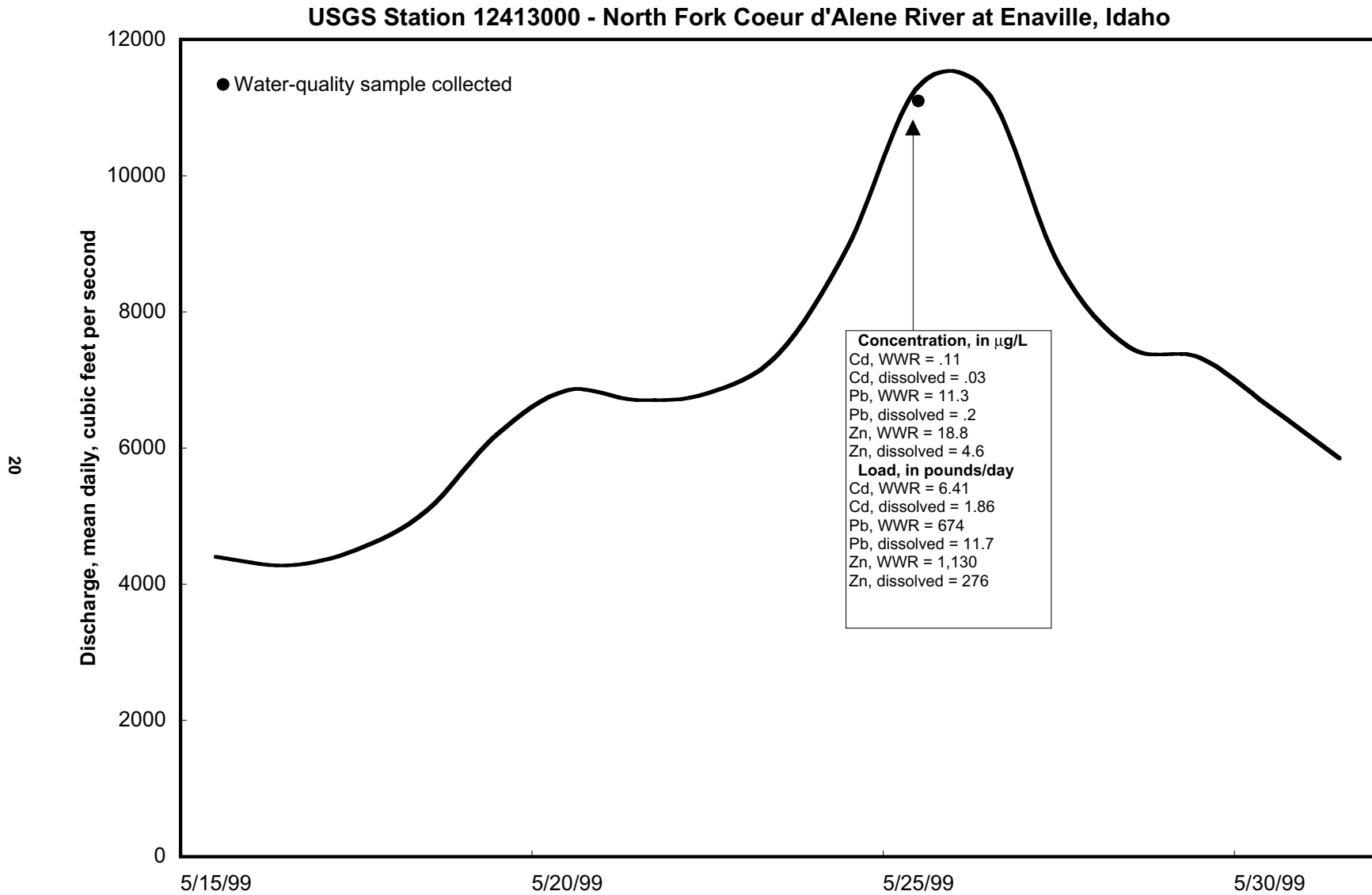
Figure 12. Near-peak portion of 1999 snowmelt-runoff hydrograph with concentrations and loads of cadmium, lead, and zinc at North Fork Coeur d'Alene River at Enaville, Idaho. (USGS, U.S. Geological Survey; \mu\text{g/L} , micrograms per liter; WWR, whole-water recoverable)
