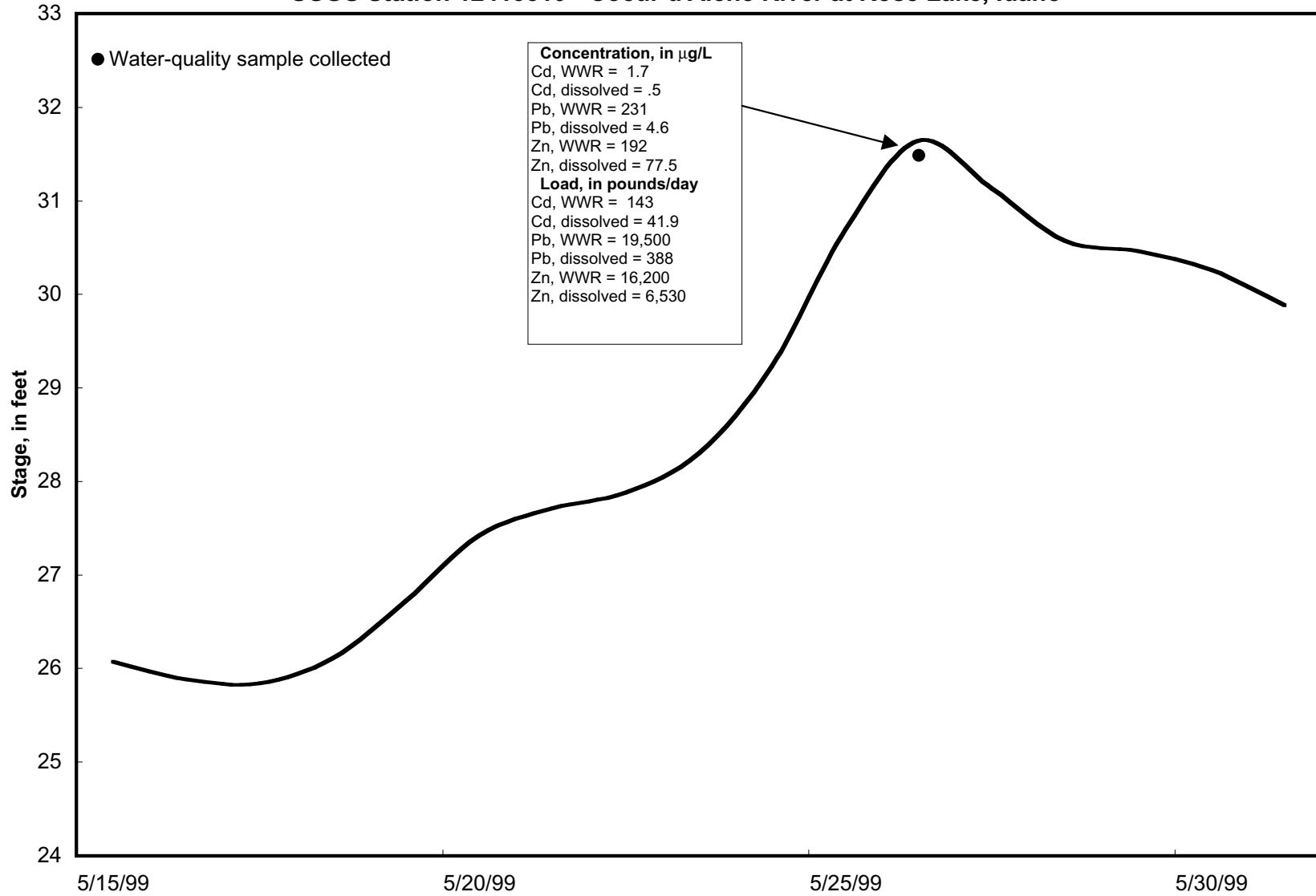
Figure 14. Near-peak portion of 1999 snowmelt-runoff hydrograph with concentrations and loads of cadmium, lead, and zinc at Coeur d'Alene River at Rose Lake, Idaho. (USGS, U.S. Geological Survey; \mu\text{g/L} , micrograms per liter; WWR, whole-water recoverable)
