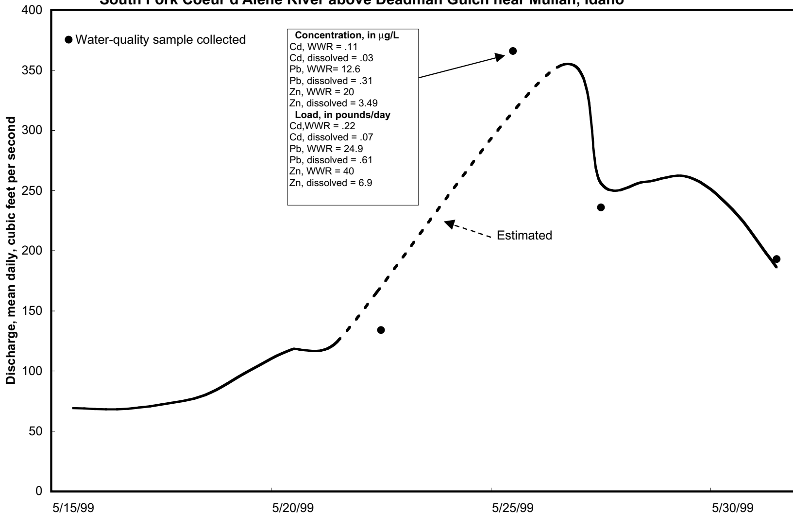
Figure 2. Near-peak portion of 1999 snowmelt-runoff hydrograph with concentrations and loads of cadmium, lead, and zinc at South Fork Coeur d'Alene River above Deadman Gulch near Mullan, Idaho. (USGS, U.S. Geological Survey; \mu\text{g/L} , micrograms per liter; WWR, whole-water recoverable)
