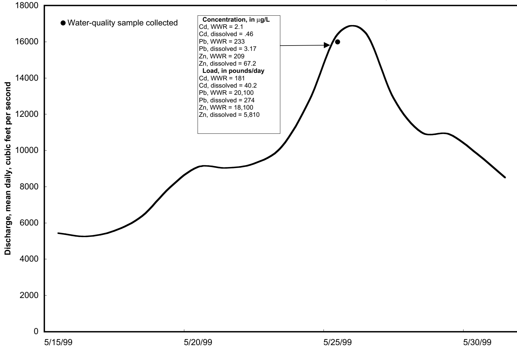
Figure 13. Near-peak portion of 1999 snowmelt-runoff hydrograph with concentrations and loads of cadmium, lead, and zinc at Coeur d'Alene River near Cataldo, Idaho. (USGS, U.S. Geological Survey; \mu\text{g/L} , micrograms per liter; WWR, whole-water recoverable)
