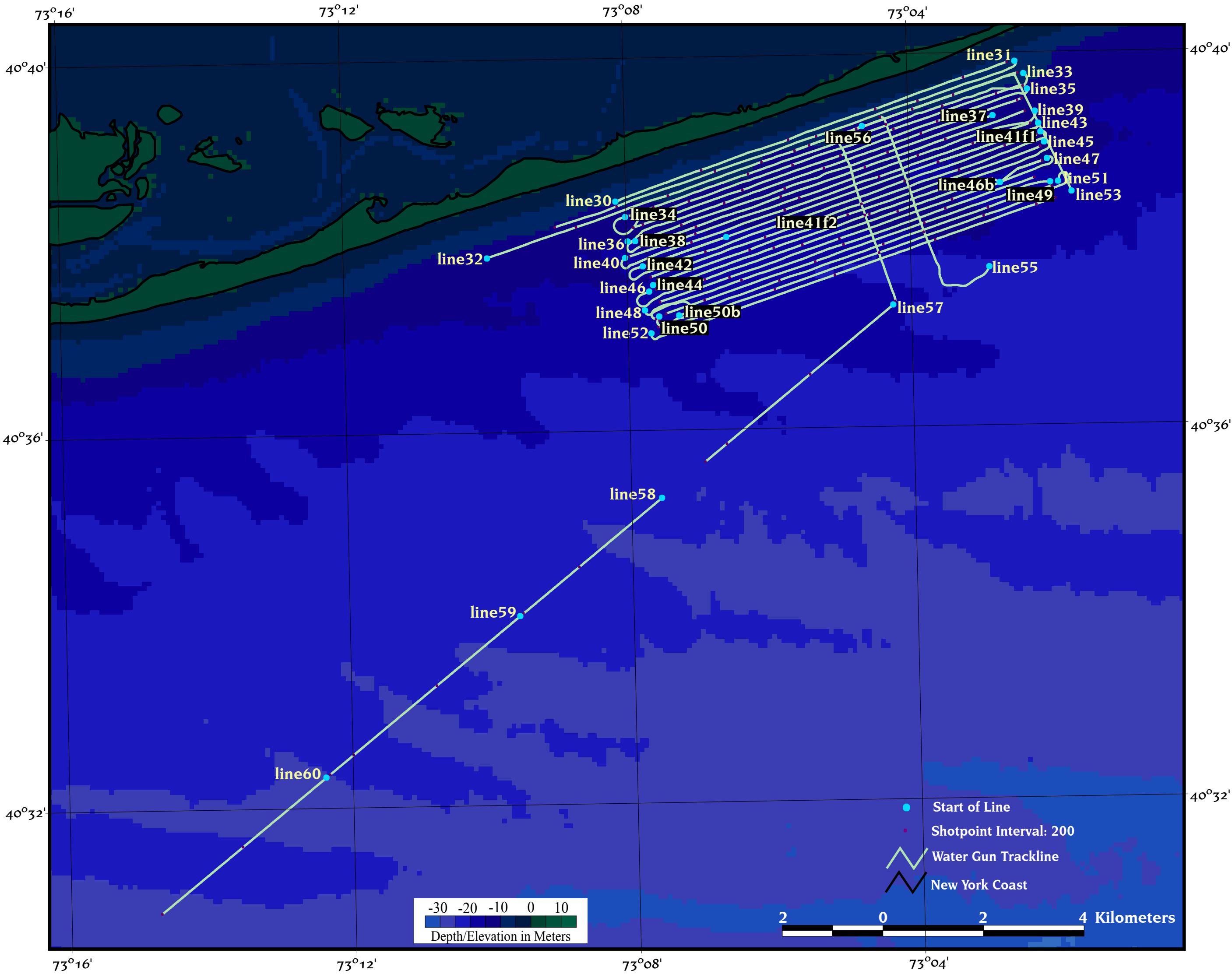
SEAX 96004 Fire Island Water Gun Survey Area (Lines 30-60)
