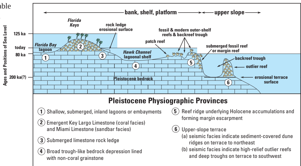
Figure 1. Schematic cross section (not to scale) showing the six general bedrock provinces along the South Florida shelf and terminology used in text. The Pleistocene ranges from ~1.77 Ma to 10 ka. The Holocene ranges from 10 ka to the present. Sea-level positions and timing shown in years before present. If sea level were to rise from its present position by 5 to 7 m, it is very likely that framework-building corals would once again become established on those areas of the Florida Keys that are basically sediment free.
