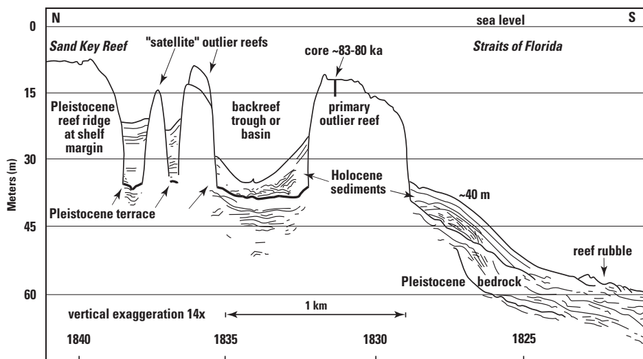
Figure 3. Interpreted seismic profile shown in Figure 2. Largest outlier reef developed at seaward edge of broad erosional surface (Pleistocene terrace). Note terrace surface is not visible beneath the reefs. Coral reefs and reef rubble or debris characteristically obscure sound-wave reflectivity of rock surfaces beneath them. A core drilled into the top of the main outlier recovered 6.09 m of coral rock. Uranium-thorium dating yielded ages of 83 to 80 ka for corals in the core. Tick marks at bottom of interpreted profile indicate time (24-hr scale).
