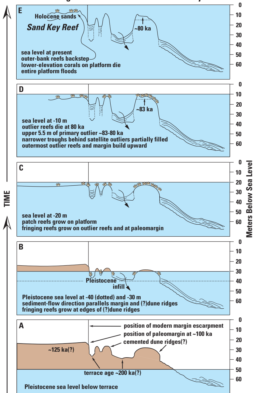
Figure 4. Proposed model for evolution of lower Keys shelf margin (sea level fluctuated many times but positions correspond to events shown). (A) Formation and cementation of sand dunes on the erosional terrace surface during a sea-level lowstand. (B) Colonization of sediment-free shelf-margin reef and dune ridges by corals. (C,D) Upward building of margin reef and outlier reefs over time and through numerous rises and falls of sea level. (E) Final demise of Pleistocene corals on outliers at ~80 ka and later migration of younger (~7- to 2-ka) outer-shelf reefs with shelf-wide flooding. Essentially no corals are alive on the outliers today. However, if sea level were to fall by some 10 m or so, it is very likely that framework-building corals would once again become established on the hard rock surface of the outlier reefs.
