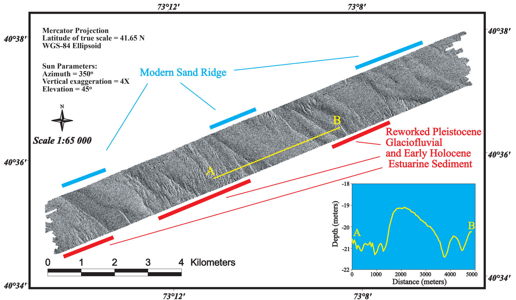
Figure 6b. Simrad EM 1000 Echo Sounder shaded relief image of the shoreface-attached sand ridges west of Watch Hill. Bathymetric profile from A to B is displayed in the insert. See Figure 2b for location.
