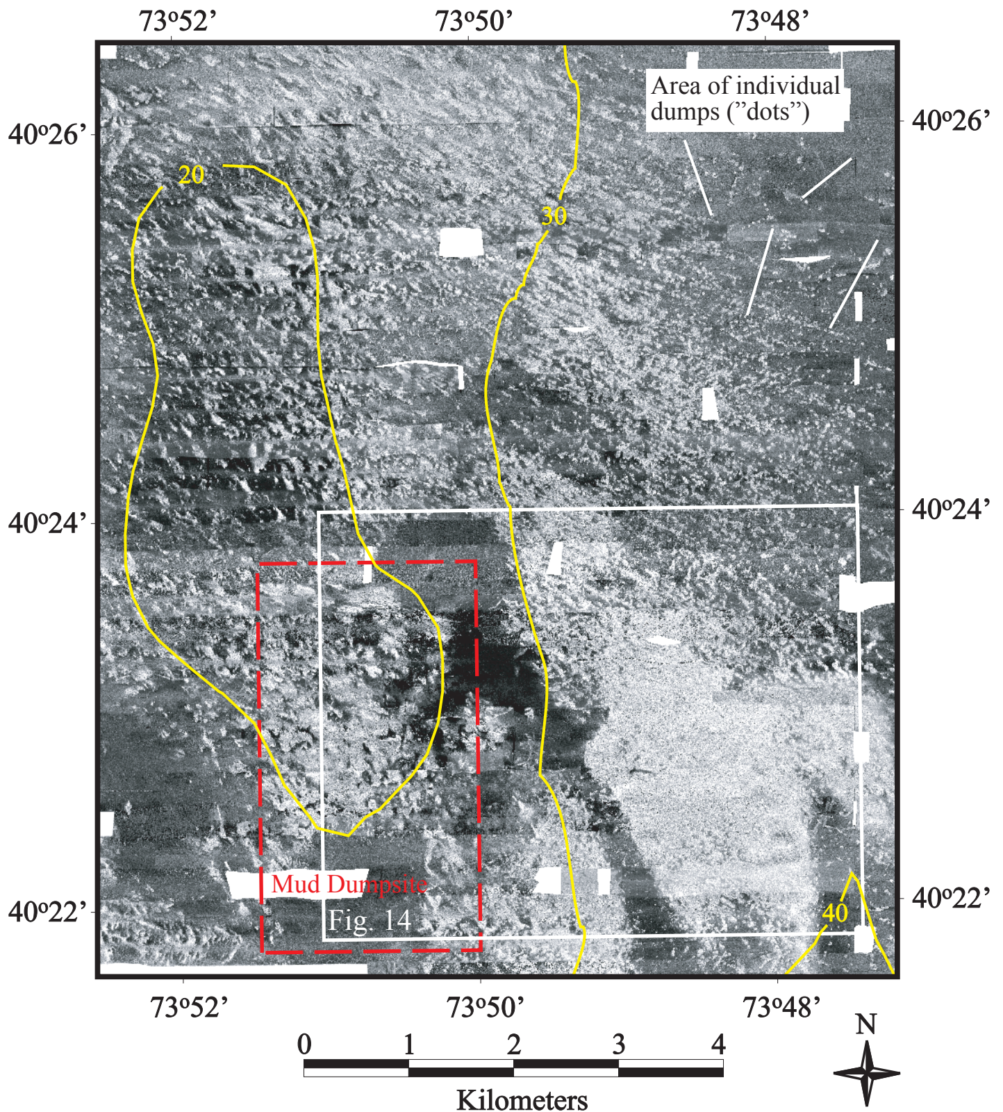
Figure 13. Sidescan-sonar image of the Mud Dumpsite area located at the head of the Hudson Shelf Valley. This area is marked by a series of high-backscatter “dots”, interpreted to be individual dumps of dredged and other material disposed in this area since the late 1800’s (arrows point to example of “dots”). High backscatter is represented by light tones, low backscatter by dark tones. Bathymetric contours are in meters. See Figure 3 for location.
