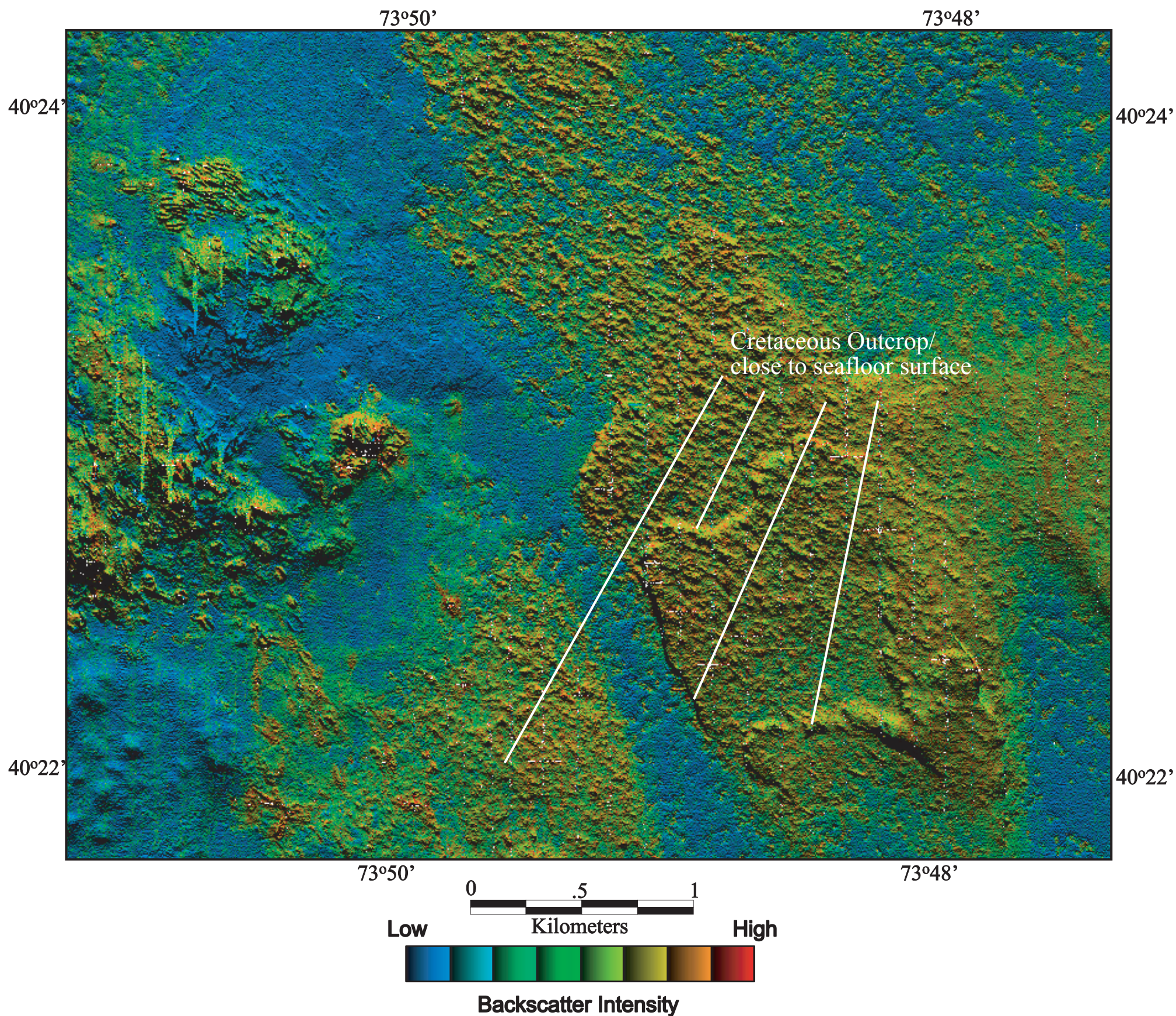
Figure 14. Simrad EM-1000 multibeam echo sounder pseudo-color backscatter image of Mud Dumpsite area located at the head of the Hudson Shelf Valley. See Figures 3 and 13 for location. Areas where Cretaceous to early Tertiary coastal plain strata crop out, or are close to the sea-floor surface, are shown.
