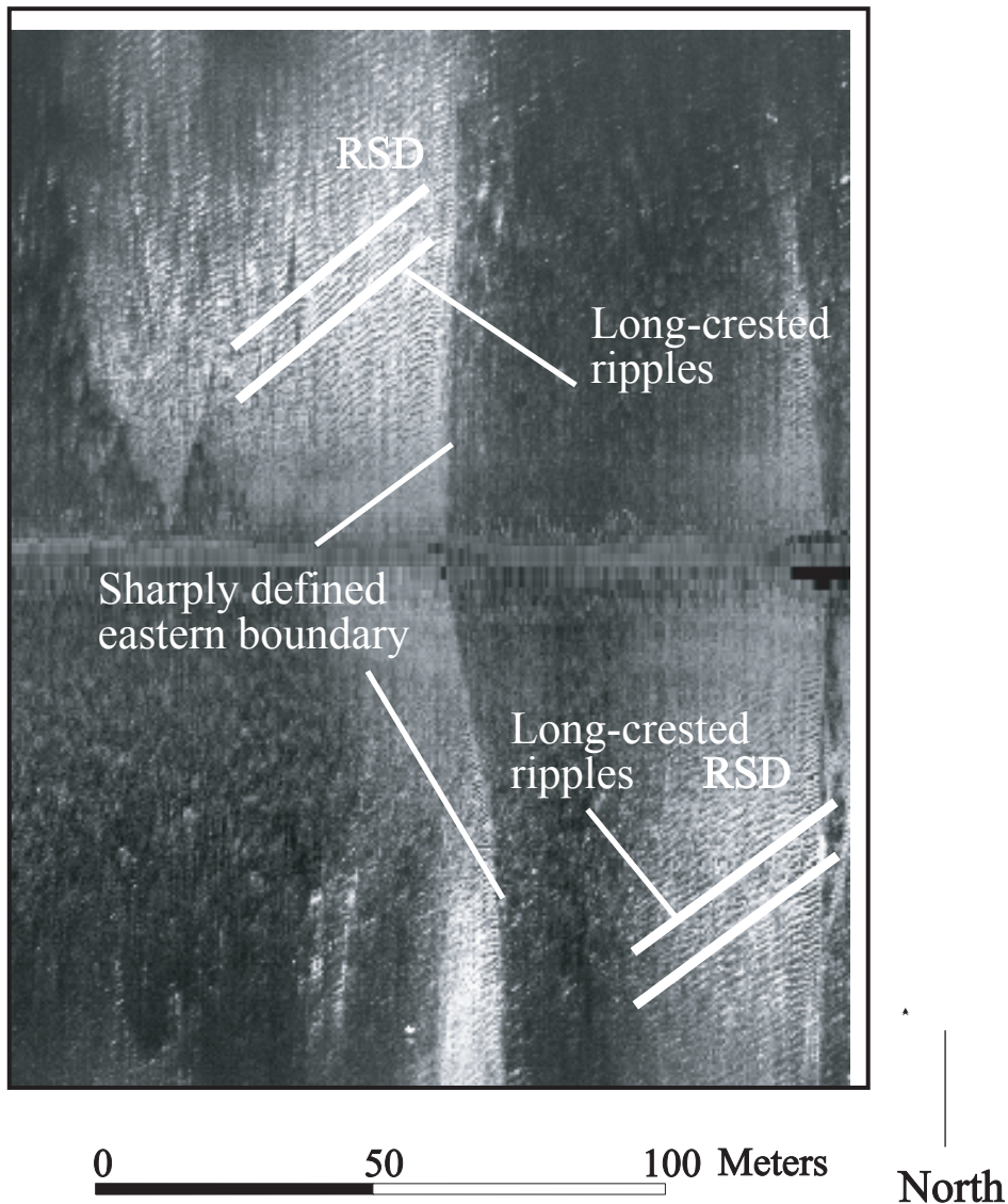
Figure 7. Enlarged image of two rippled scour depressions showing the long-crested ripples which floor the high-backscatter depressions. Ripple crests are oriented roughly shore-parallel, as illustrated by the white lines. The sharply defined eastern boundaries of the high-backscatter areas are also displayed. See Figure 6 for location.
