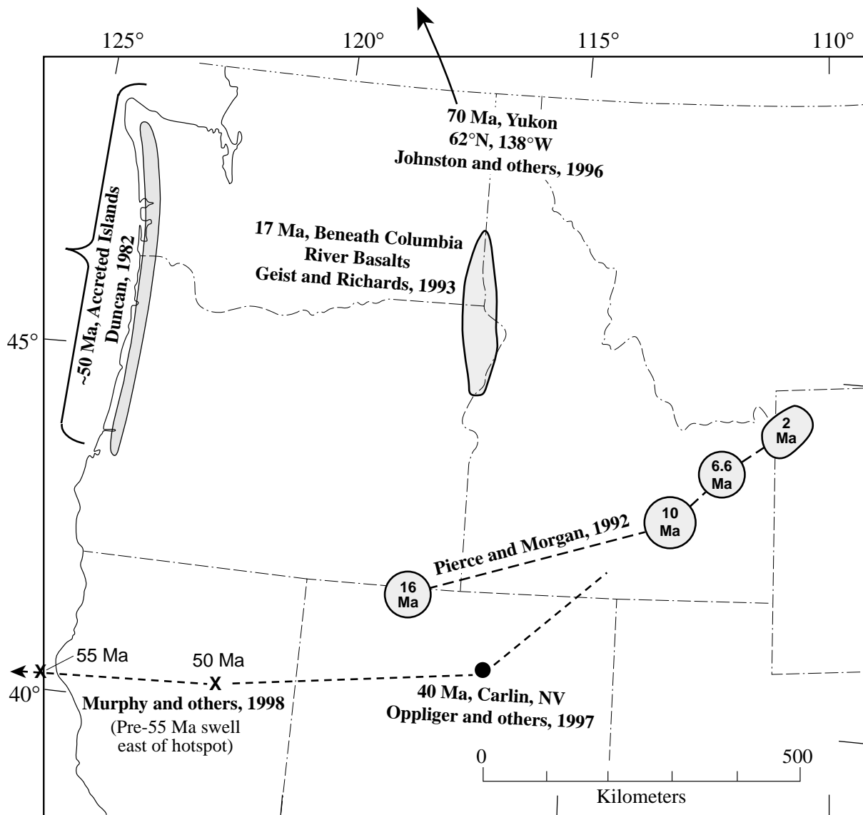
Figure 4. Some positions for the Yellowstone hotspot at different times as postulated by others and by us. The location between 50 and 17 Ma presents a problem that is avoided if the Yellowstone plume starts at 17 Ma.
