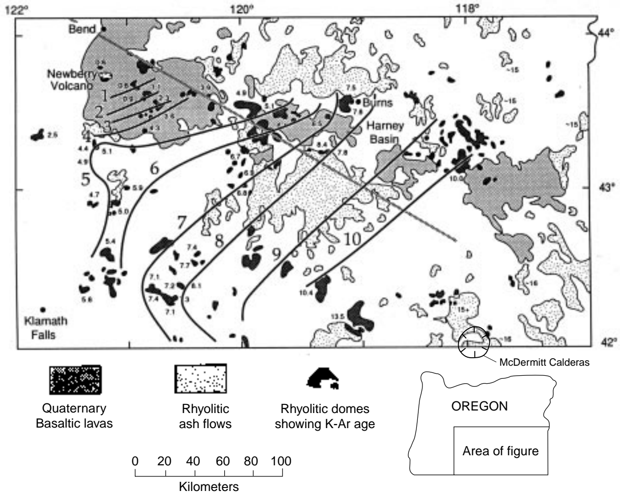
Figure 7. Age progression of silicic lava domes of the southern Oregon rhyolite belt. This figure shows upper Miocene and younger volcanic rocks and is copied from Christiansen and Yeats (1992, fig. 55). The rhyolite domes and their ages were shown by MacLeod and others (1976) to have such a systematic northwest decrease in age that ages could be contoured in one-million-year increments. This northwest age progression is a key argument against a plume origin for the Yellowstone hotspot (Lipman, 1992; Christiansen and Yeats, 1992). See Figure 9 for our suggestions about how the southern Oregon rhyolite belt might be reconciled with a thermal plume origin of the Yellowstone hotspot. Both the southern Oregon rhyolite belt and the Yellowstone hotspot track start in the region near McDermitt, but they become younger in nearly opposite directions at the same time. The silicic domes (dark) form two belts that trend N. 75° W. The northern belt ends at Newberry caldera and parallels the Brothers fault zone (wide gray line) which is actually a complex en echelon pattern of normal faults whose trend of about 10° clockwise to the overall pattern (Walker and Nolf, 1981) suggests a right lateral component (Pezzopane and Weldon, 1993). Between 10 and 17 Ma, ignimbrites and other silicic volcanism are widespread in the southern Oregon, northern Nevada and southwestern Oregon area (fig. 1; Pierce and Morgan, 1992); but have no systematic progression with age in southeast Oregon (MacLeod and others, 1976, p. 470).
