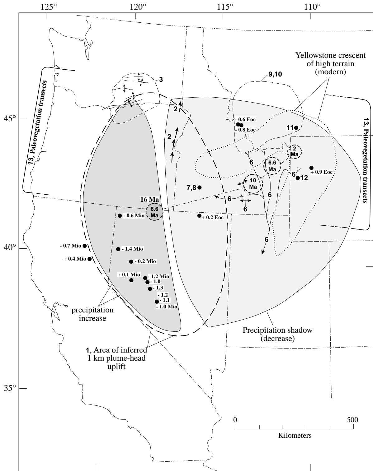
Figure 9. Uplift and climatic patterns that may relate to Yellowstone plume (both head and tail). The dashed line shows the pancaked plume with a diameter suggested by Parsons and others (1994) of about 400 km but elongated north south as suggested by Camp (1995) parallel to the Nevada-Oregon rift zone. Table 1 describes the various localities, areas, and transects shown here. One of the main climatic parameters listed is orographic dryness (light shading) in the lee of the inferred Yellowstone plume-head uplift. In general, observations of uplift and climate are compatible with uplift above the plume head followed by uplift migrating to the east associated with the plume tail (chimney) to the "Yellowstone crescent of high terrain" associated with the present plume tail (Pierce and Morgan, 1992) or a similar 650-m-high altitude anomaly that Smith and Braille (1993) associated with the current Yellowstone hotspot.
