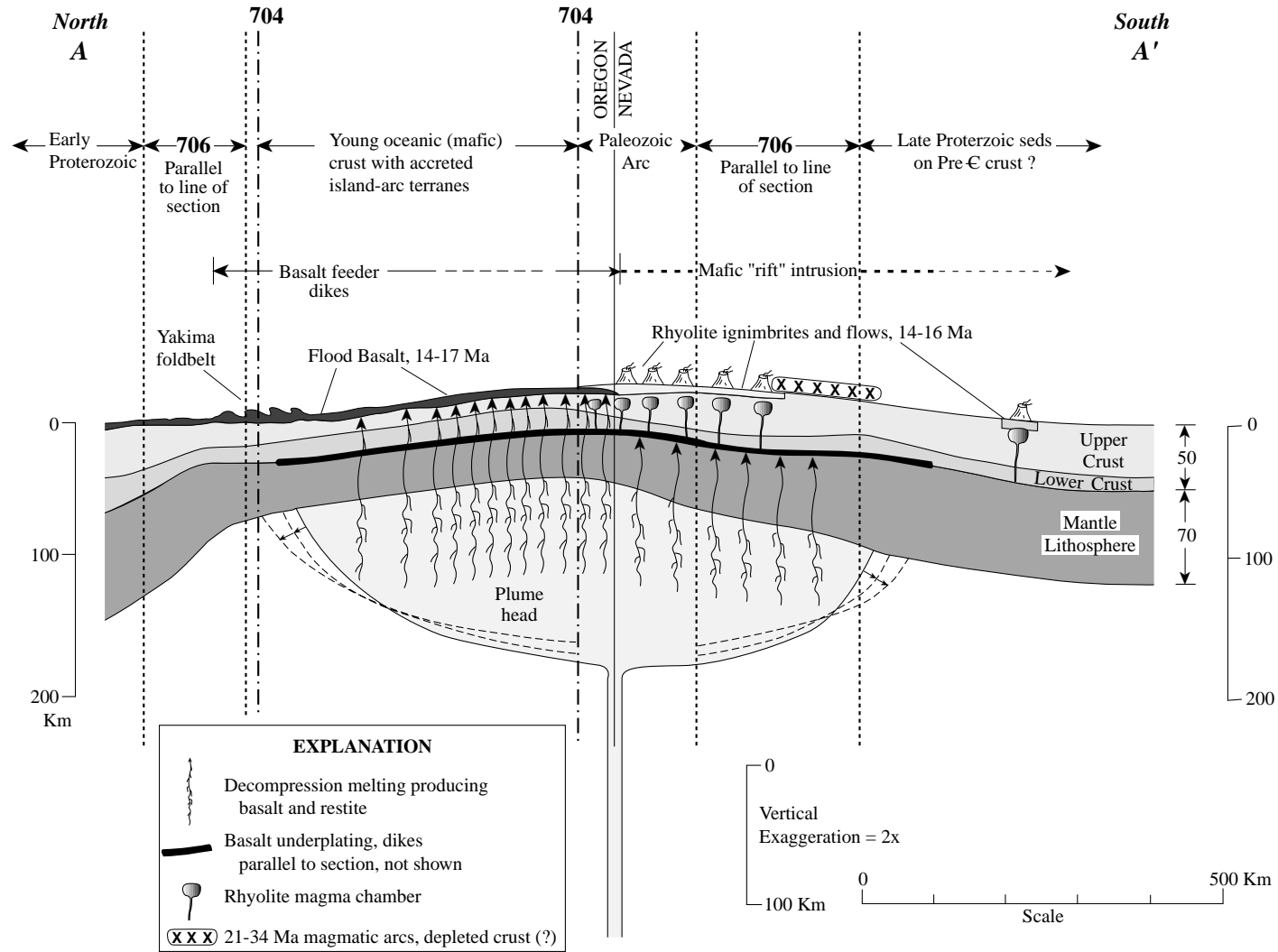
Figure 6. Geologic cartoon along line of section A-A' showing emplacement of postulated Yellowstone plume head. The plume head spreads out (pancakes, mushrooms) upon rising into the lithosphere, but it can rise further beneath the thinner lithosphere (young thin mafic crust and lithospheric mantle) beneath Oregon. Decompression melting (squiggly vertical lines) produces basalt magma that rises upward and interacts differently with the crust: (A) in Oregon, magma rises through the dense, more oceanic crust, and surfaces as the Columbia River and Oregon Plateau flood basalts, and (B) in Nevada and southern Oregon, basalt magma melts silicic lower crustal material that then rises into upper crust forming magma chambers (oval pods) and rhyolitic ignimbrite eruptions, shown as volcanoes, and (C) in northernmost Nevada and southern Oregon, both processes have operated. The restite from decompression melting remains in the mantle but is buoyant and contributes to long-lasting uplift (Morgan and others, 1995). At the time of emplacement, doming above the plume head may be 1-2 km (exaggerated in drawing). The northward gravitational push from this doming may have produced the Yakima fold belt near the northern end of the section.
