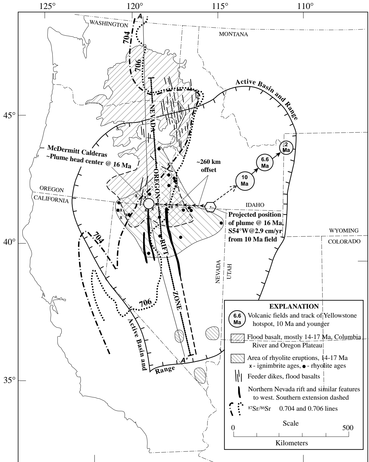
Figure 1. Map of western United States showing the track of the Yellowstone hotspot (after Pierce and Morgan, 1992, fig. 23). The 10- to-2-Ma track is compatible with plate motion, whereas the 10- to-16-Ma track has apparent rates three times faster than predicted. Projecting back from 10 Ma, we infer the plume was located at the site of the hexagon. As shown by the arrowed line, the geologic location of the inferred plume head was about 260 km further west at about the McDermitt caldera. Assuming the Vancouver slab was in the subsurface (figs. 2 and 3), buoyant rise up the slab may have deflected the plume head westward the 260 km shown by the arrowed line. Strontium lines after Reed (1993) with modifications in Washington from Robert Fleck (written commun., 1998) and southeastern Idaho from Leeman and others (1992). Transect A-A' is portrayed in Figure 5.
