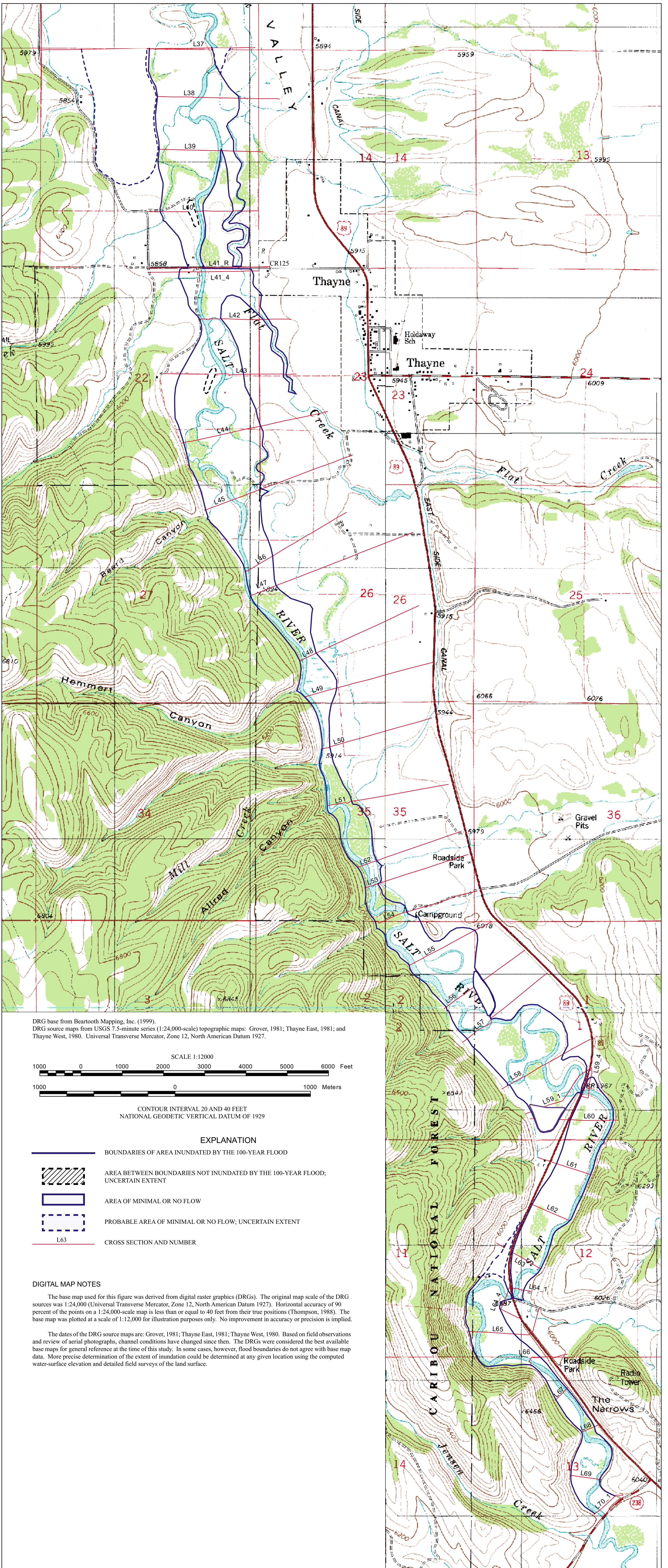
Figure 9. Locations of surveyed cross-sections and flood boundaries for the computed 100-year flood, lower Salt River, Lincoln County, Wyoming.
