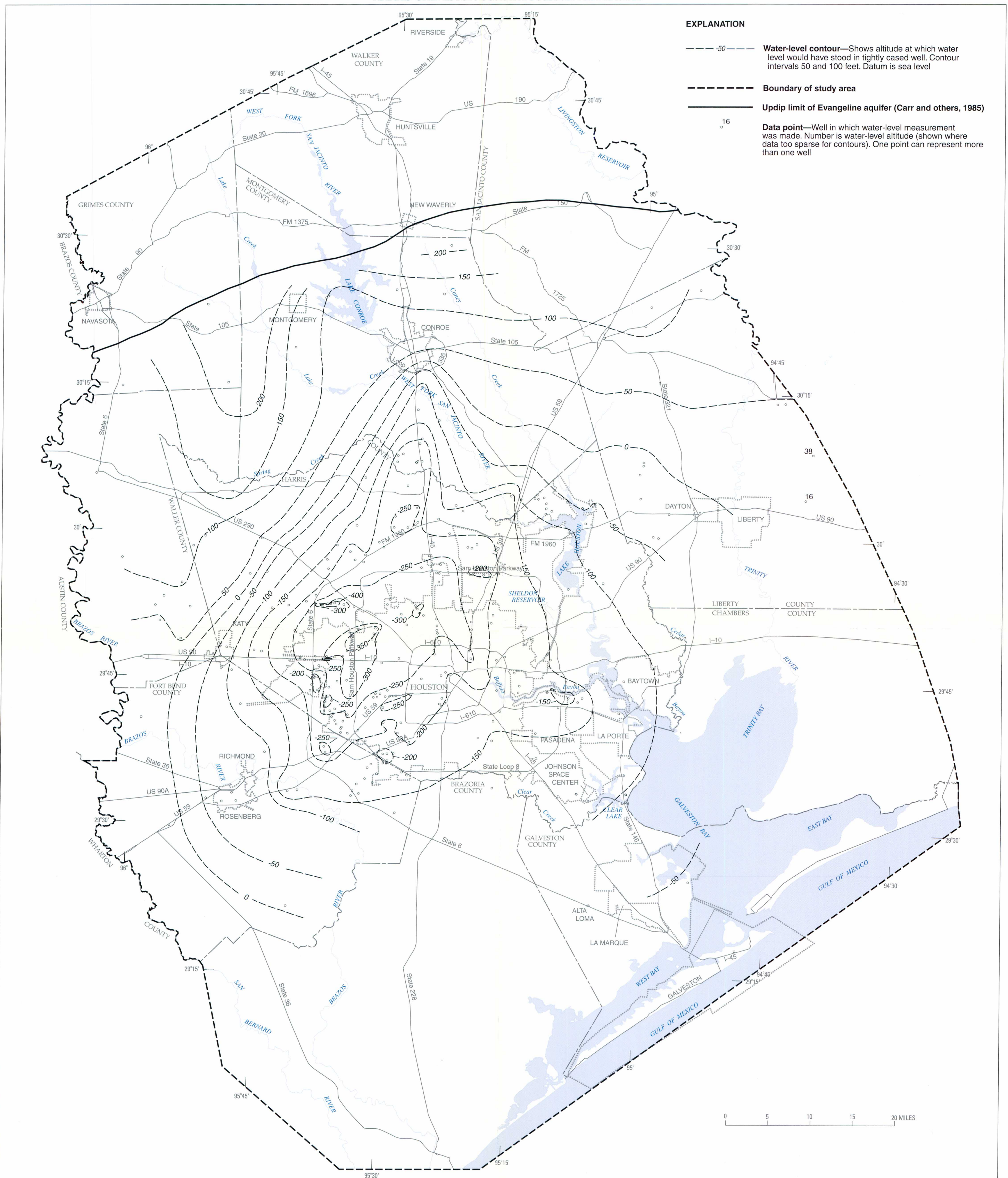
Figure 4. Map showing approximate water-level altitudes in the Evangeline aquifer, Houston-Galveston region, Texas, January–February 2001.
