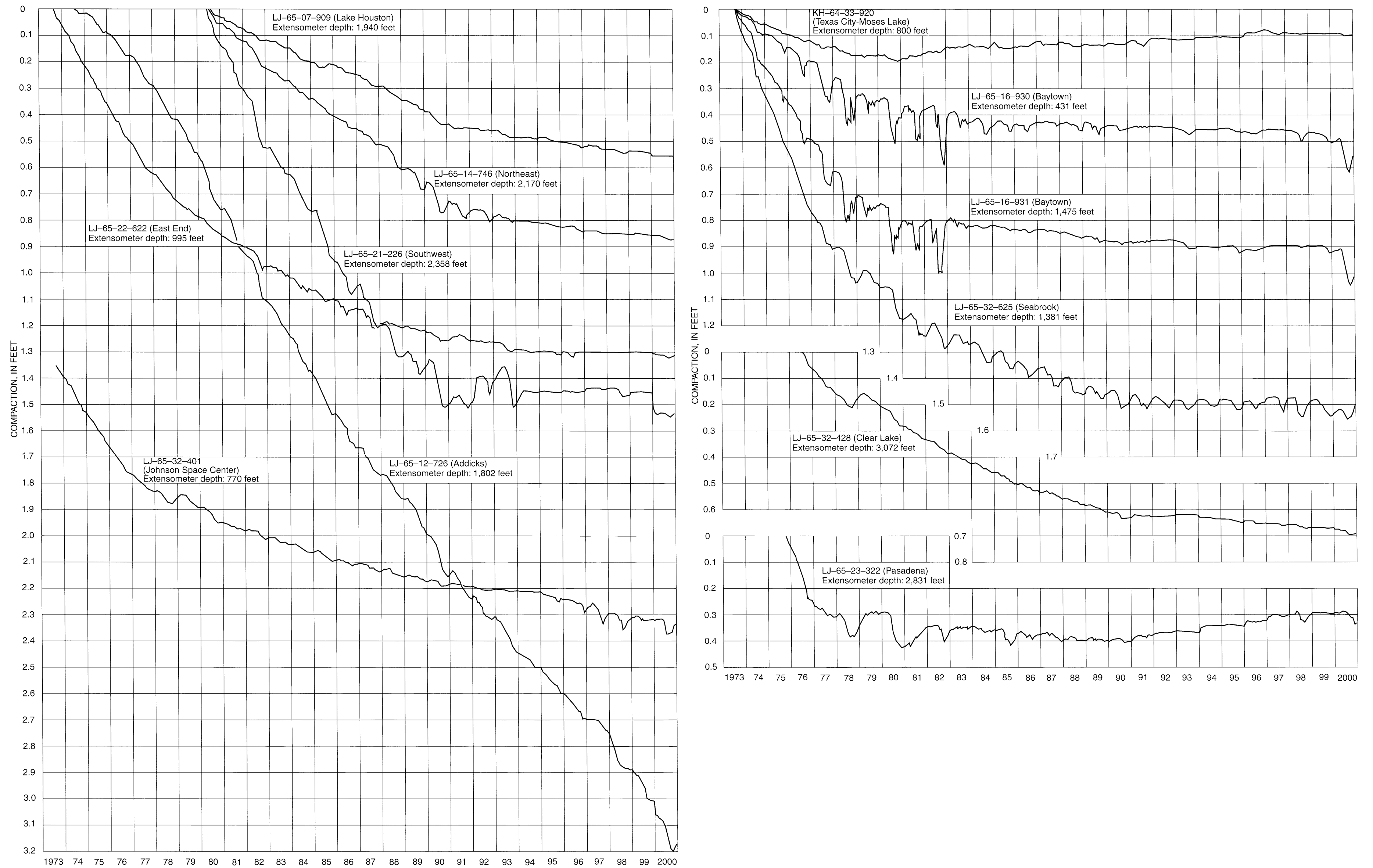
Figure 8. Graphs showing measured compaction of subsurface material, 1973-2000, at extensometer sites shown in figure 7.
