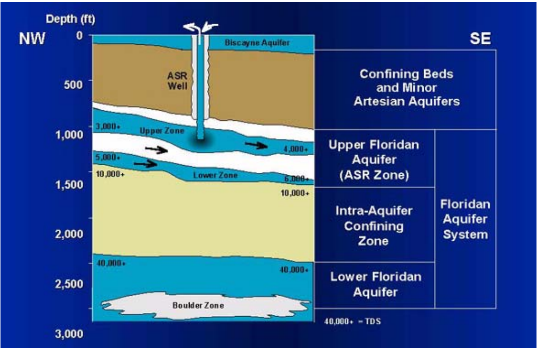
Figure 9. Conceptual hydrogeologic cross-section illustrating aquifer storage and recovery (ASR) in south Florida.
