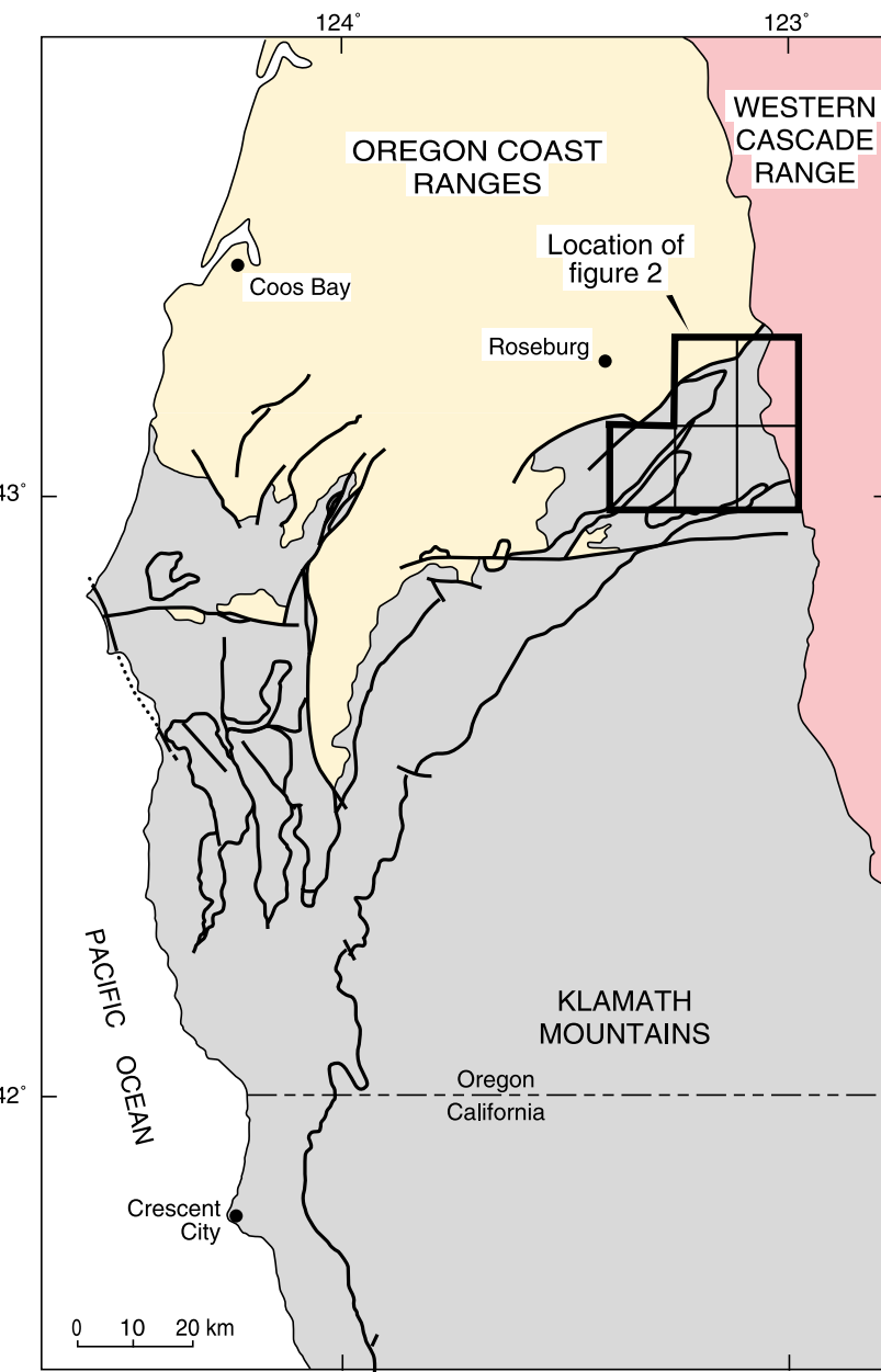
Figure 1. Location Map modified from Ryberg (1984) and Coleman and Loughery (1994).
