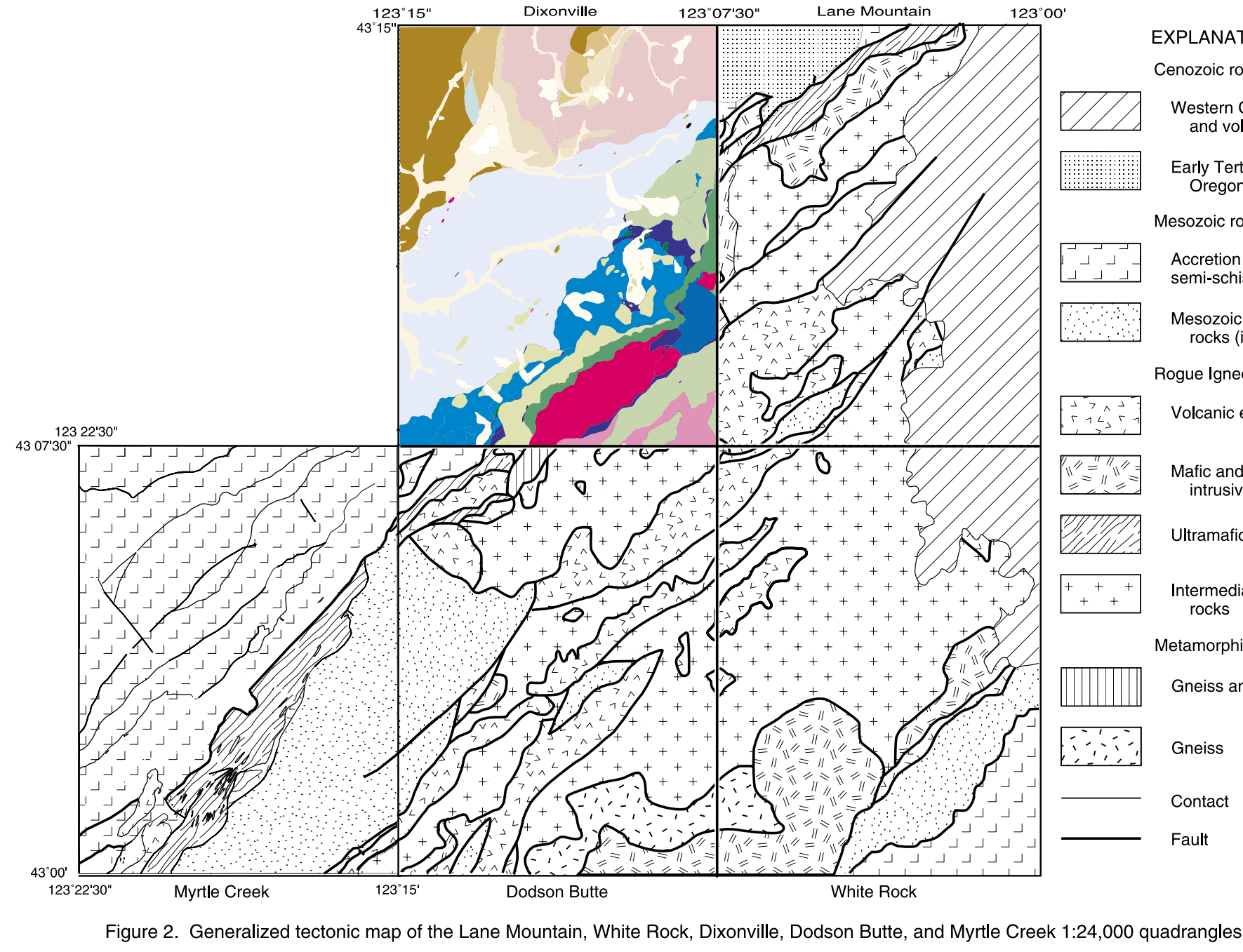
Figure 2. Generalized tectonic map of the Lane Mountain, White Rock, Dixonville, Dodson Butte, and Myrtle Creek 1:24,000 quadrangles
