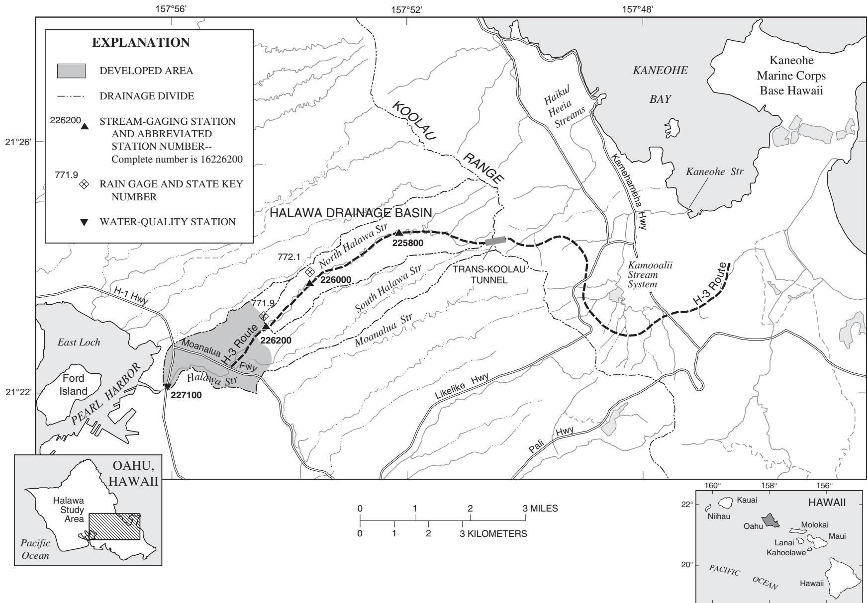
Figure 1. Selected stream-gaging stations and drainage basins in the H-3 Highway study area, Oahu, Hawaii.
