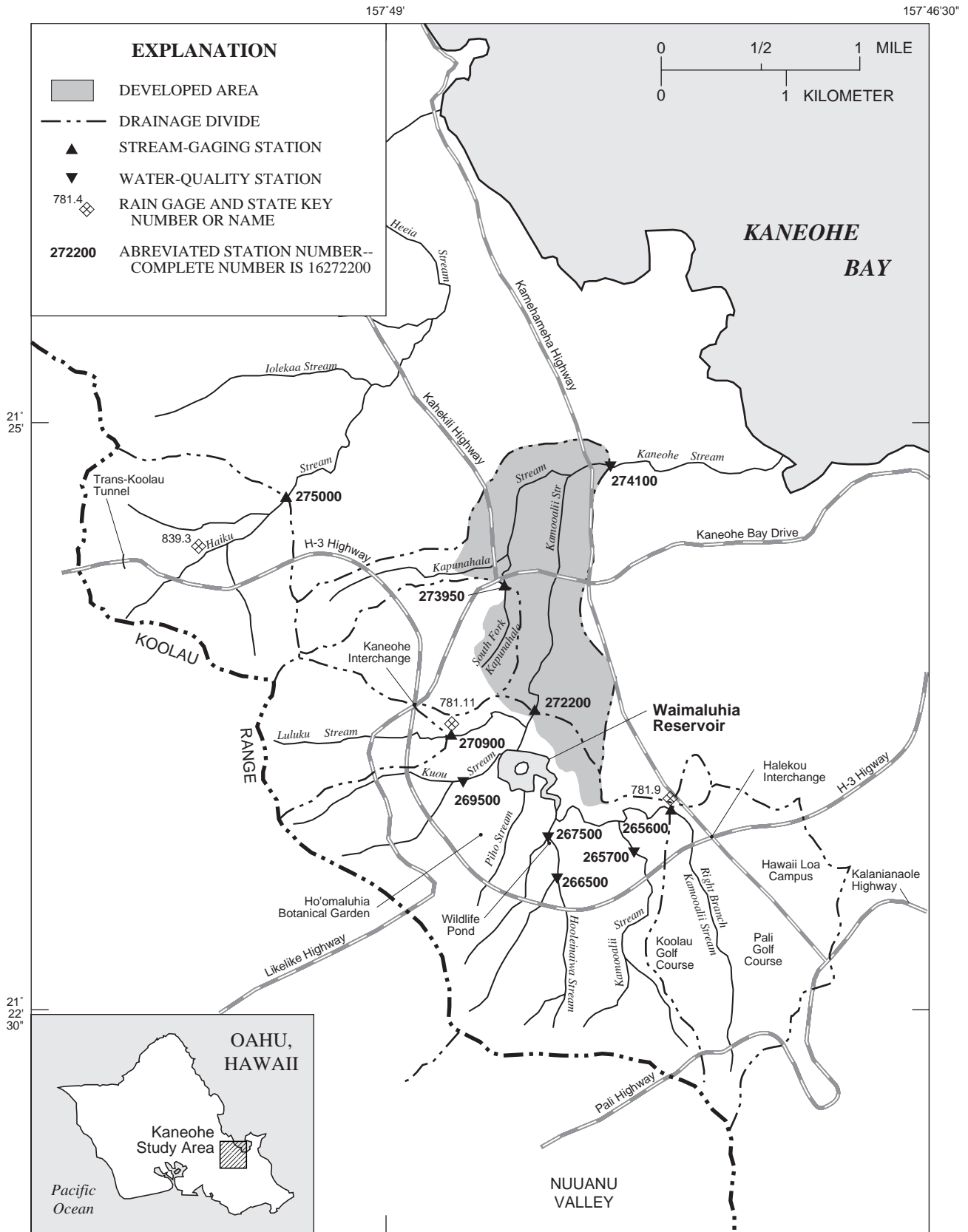
Figure 2. Haiku and Kaneohe drainage basins study area, Oahu, Hawaii.
