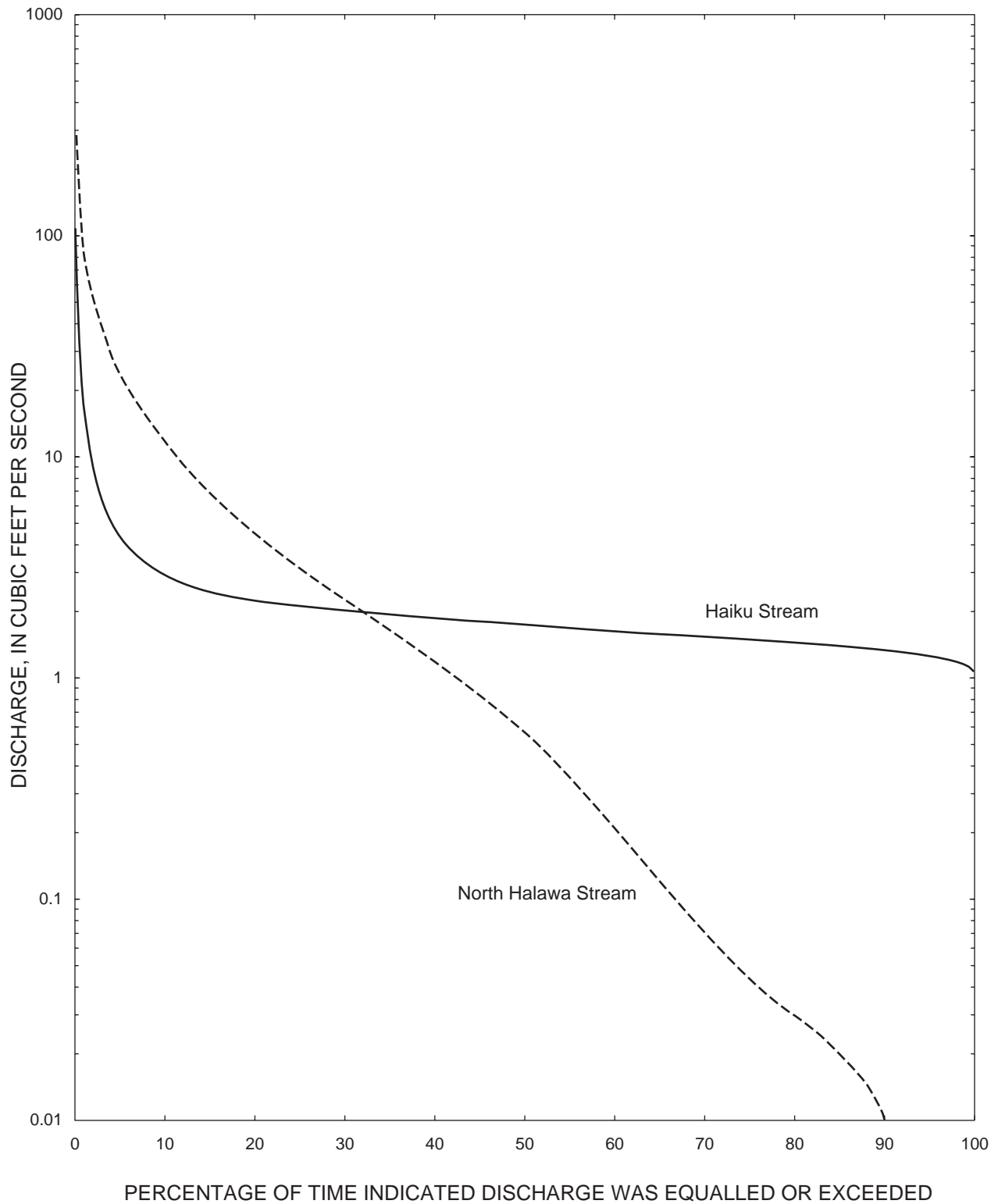
Figure 4. Flow-duration curves of daily flows for stations 16226200 North Halawa Stream and 16275000 Haiku Stream, 1983-99, Oahu, Hawaii.
