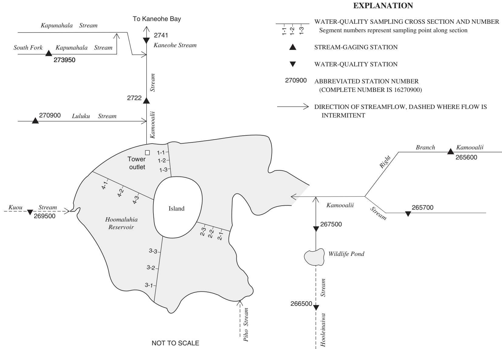
Figure 5. Diagram showing stream-gaging and water-quality stations in the Kaneohe drainage basin, Kaneohe, Oahu, Hawaii.
