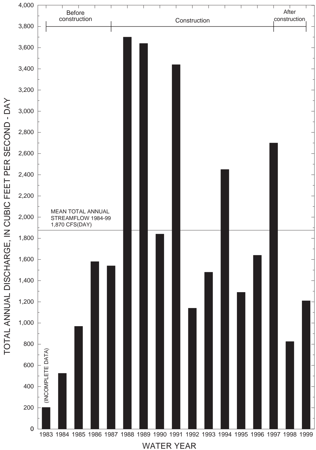
Figure 7. Total annual streamflow at station 16226200, North Halawa Stream near Honolulu, Oahu, Hawaii, water years 1983–99.
