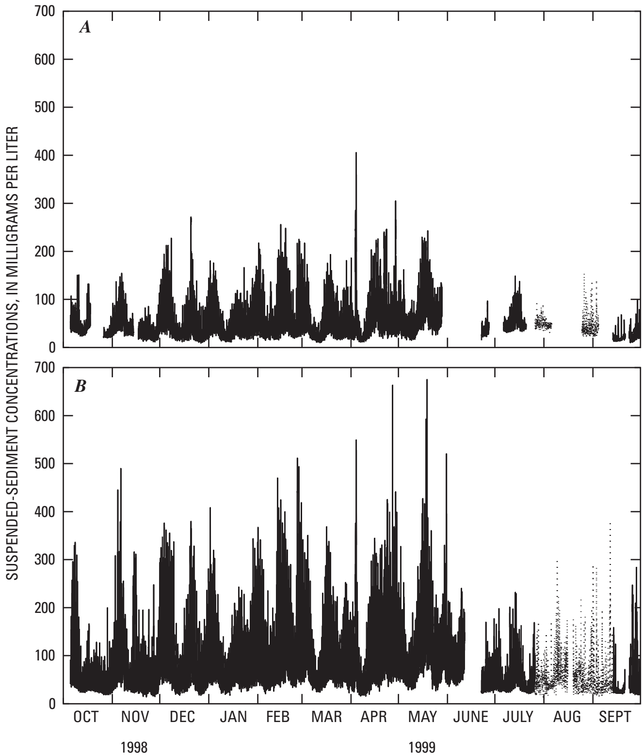
Figure 13. Time series of mid-depth ( A ) and near-bottom ( B ) suspended-sediment concentrations calculated from sensor readings at Point San Pablo, Central San Francisco Bay, California, water year 1999.
