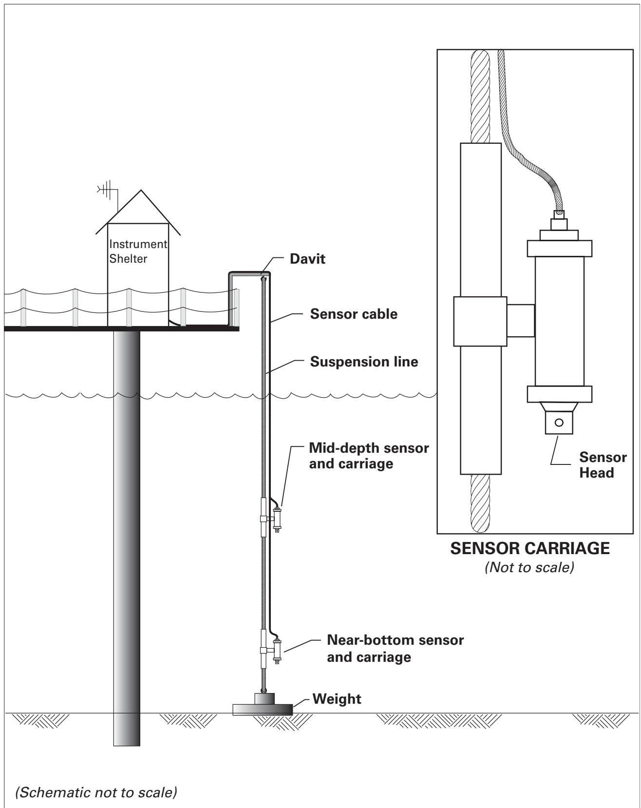
Figure 2. Monitoring installation.
