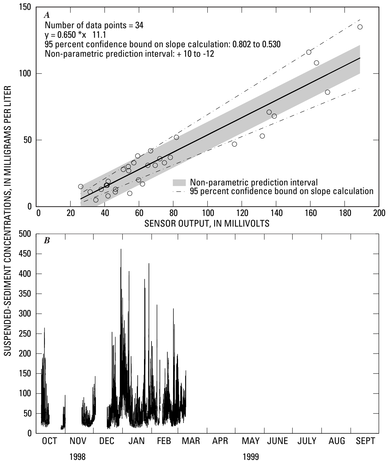
Figure 20. Calibration of mid-depth optical backscatterance sensor (A) and mid-depth suspended-sediment concentration (B) calculated from sensor readings at San Mateo Bridge, South San Francisco Bay, California, water year 1999.
