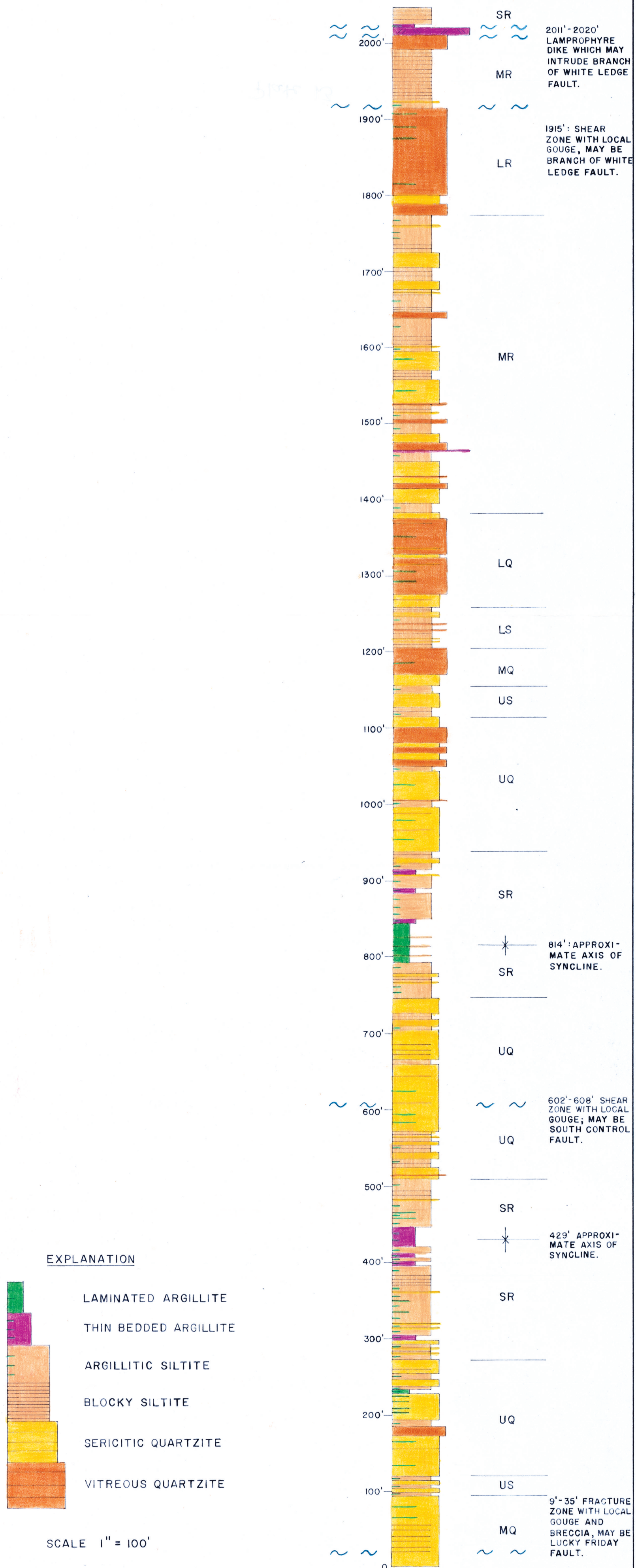
Plate 13- STRATIGRAPHY OF PART OF THE REVETT AND ST. REGIS FORMATIONS, AS EXPOSED IN ALLIED SILVER D.D.H. #83-1. DEPTH, AS MEASURED ALONG THE CORE HAS BEEN CONVERTED TRIGONOMETRICALLY TO STRATIGRAPHIC THICKNESS.
