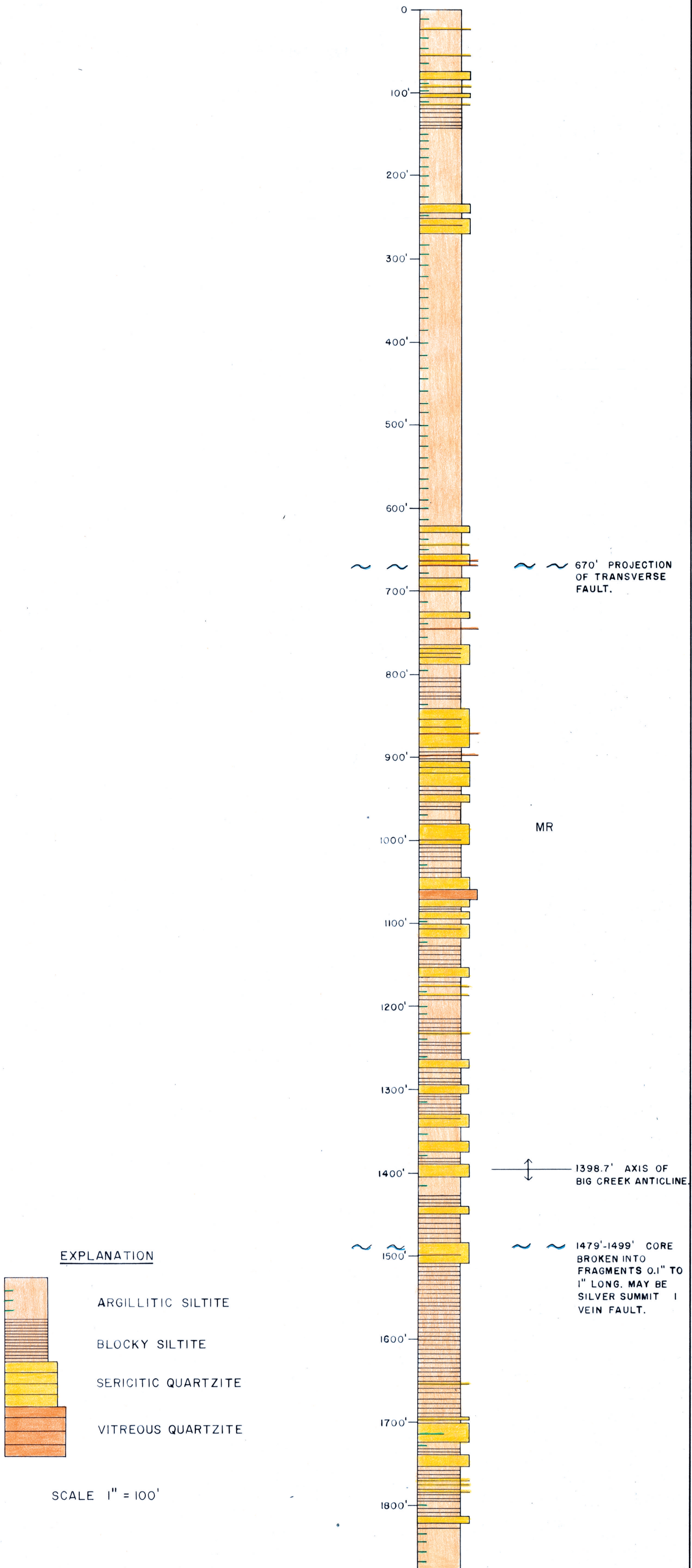
Plate 29 - STRATIGRAPHY OF PART OF THE MIDDLE REVETT, AS EXPOSED IN CON SIL DDH 54-2. DEPTH, AS MEASURED ALONG THE CORE, HAS BEEN CONVERTED TRIGONOMETRICALLY TO STRATIGRAPHIC THICKNESS.
