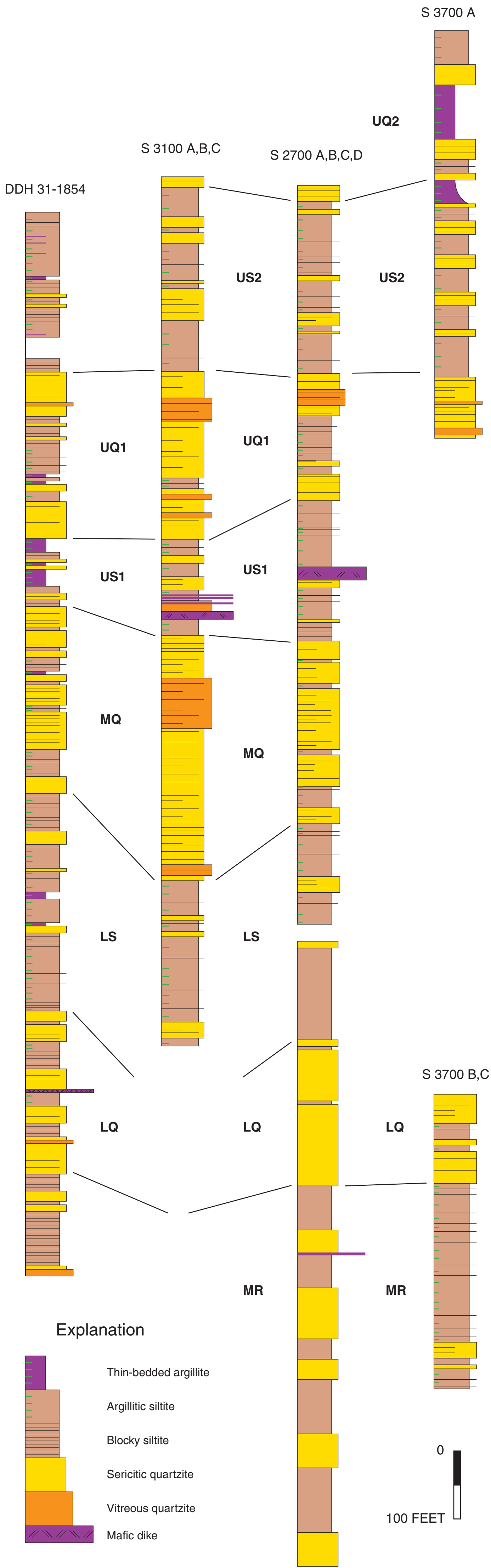
Plate 43 - Stratigraphic correlations within the Sunshine Mine
