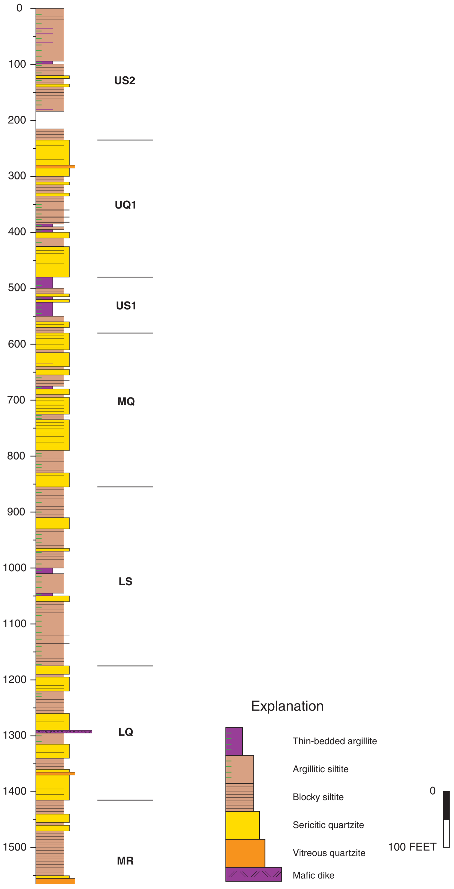
Plate 53 - Stratigraphy of part of the upper and middle Revett Fm, as exposed in Sunshine DDH #31-1854. Depth, as measured along the core, has been converted trigonometrically to stratigraphic thickness.
