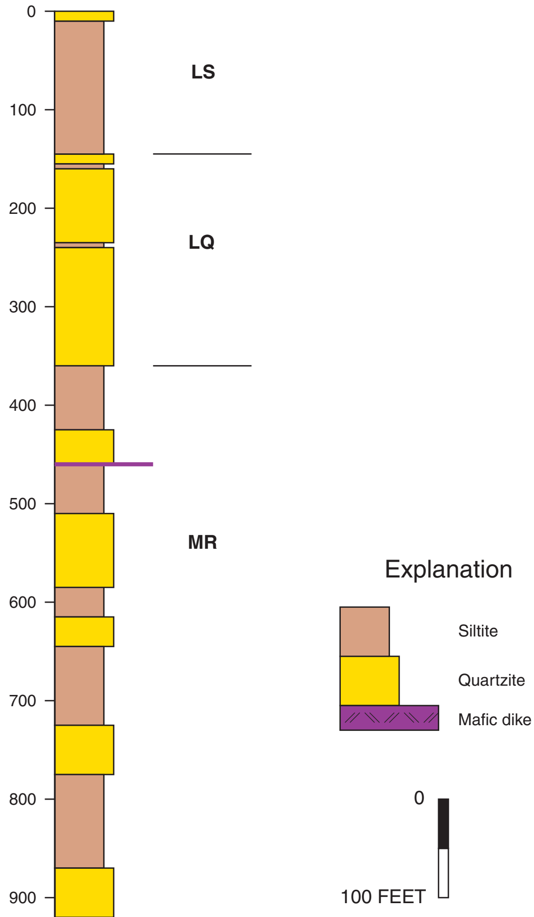
Plate 54 - Stratigraphy of part of the upper and middle Revett Fm, as exposed in the Bismark cross-cut in the Sunshine mine. Distance along the rib has been converted trigonometrically to stratigraphic thickness.
