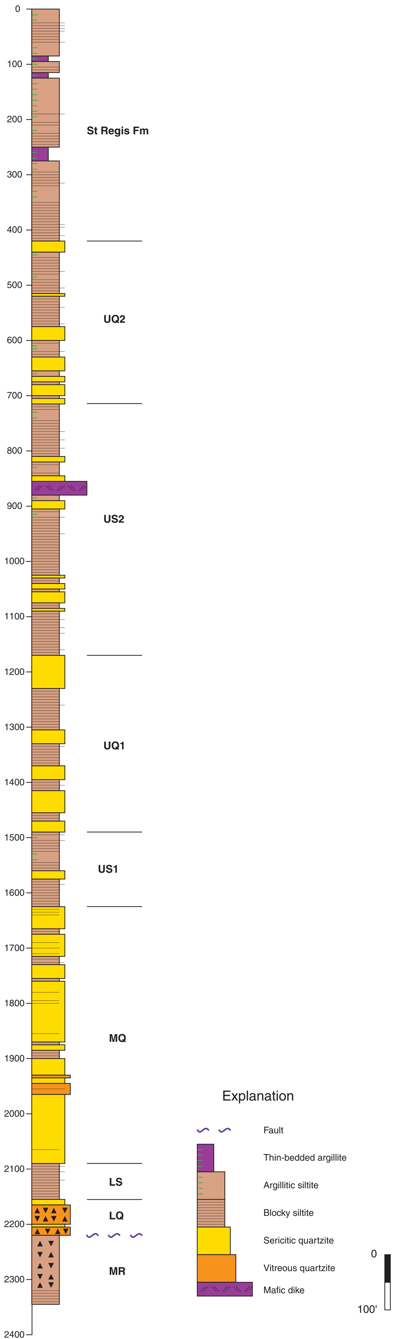
Plate 60 - Stratigraphy of part of the Revett and St Regis Formations, as exposed in Reindeer Queen DDH #85-1. Depth, as measured along the core, has been converted trigonometrically to stratigraphic thickness.
