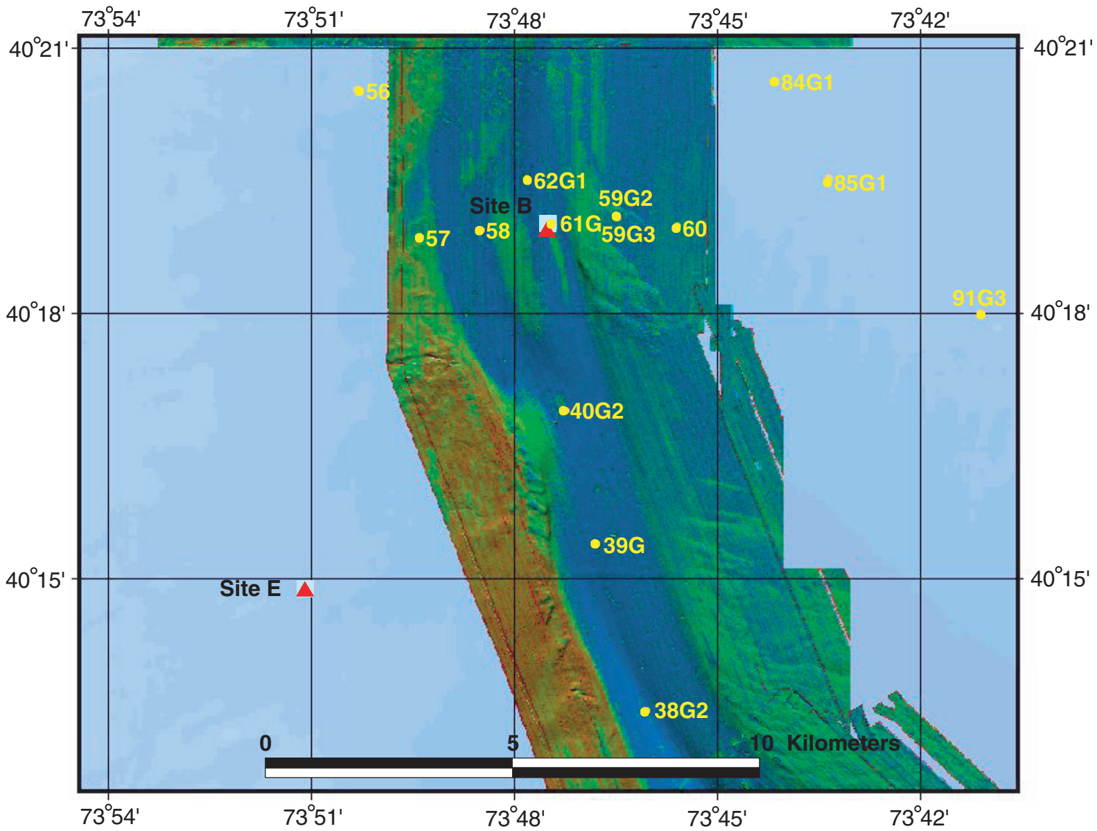
Locations of a subset of stations occupied on F/V Alpha and Omega.
