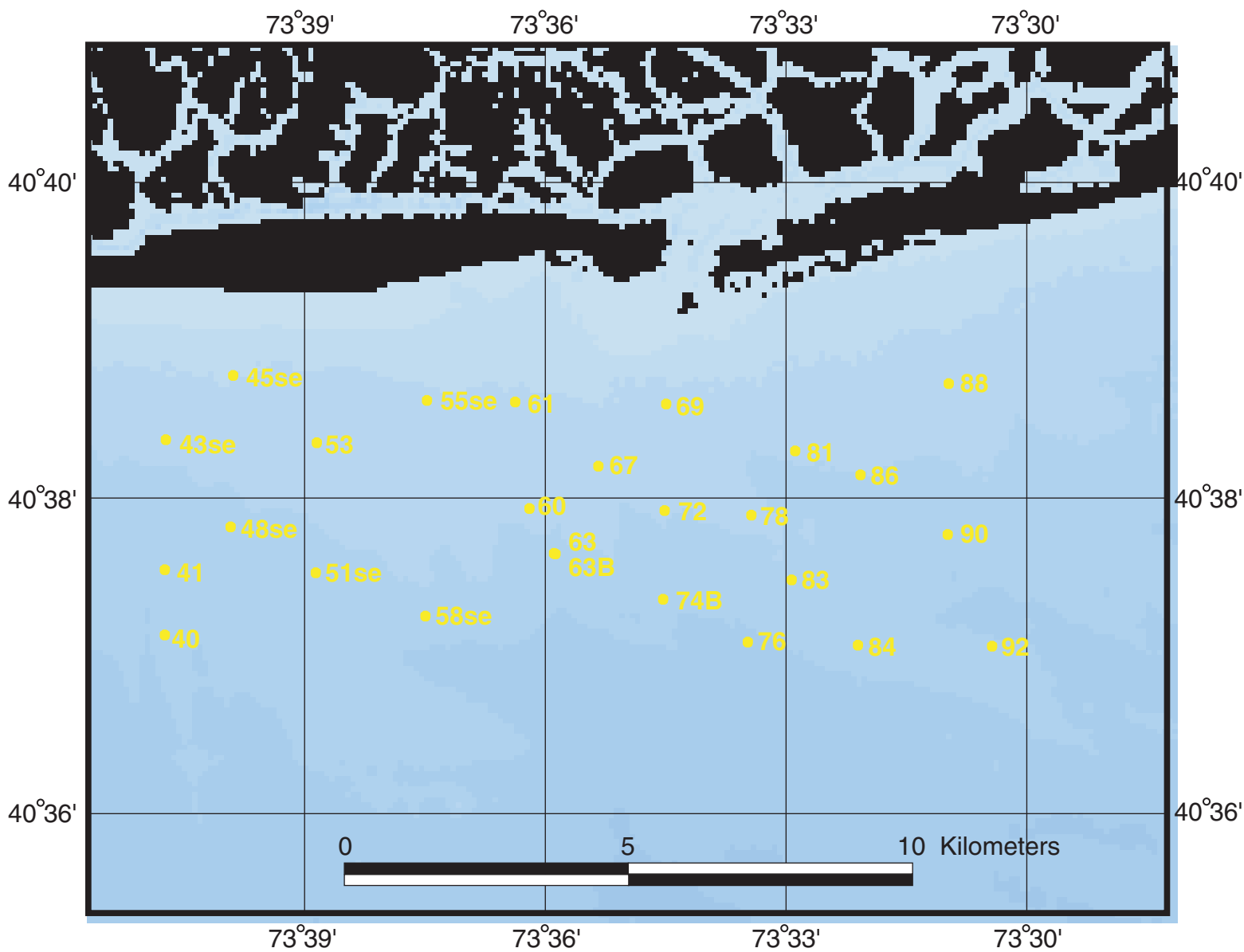
Locations of a subset of stations occupied on R/V Seward Explorer.
