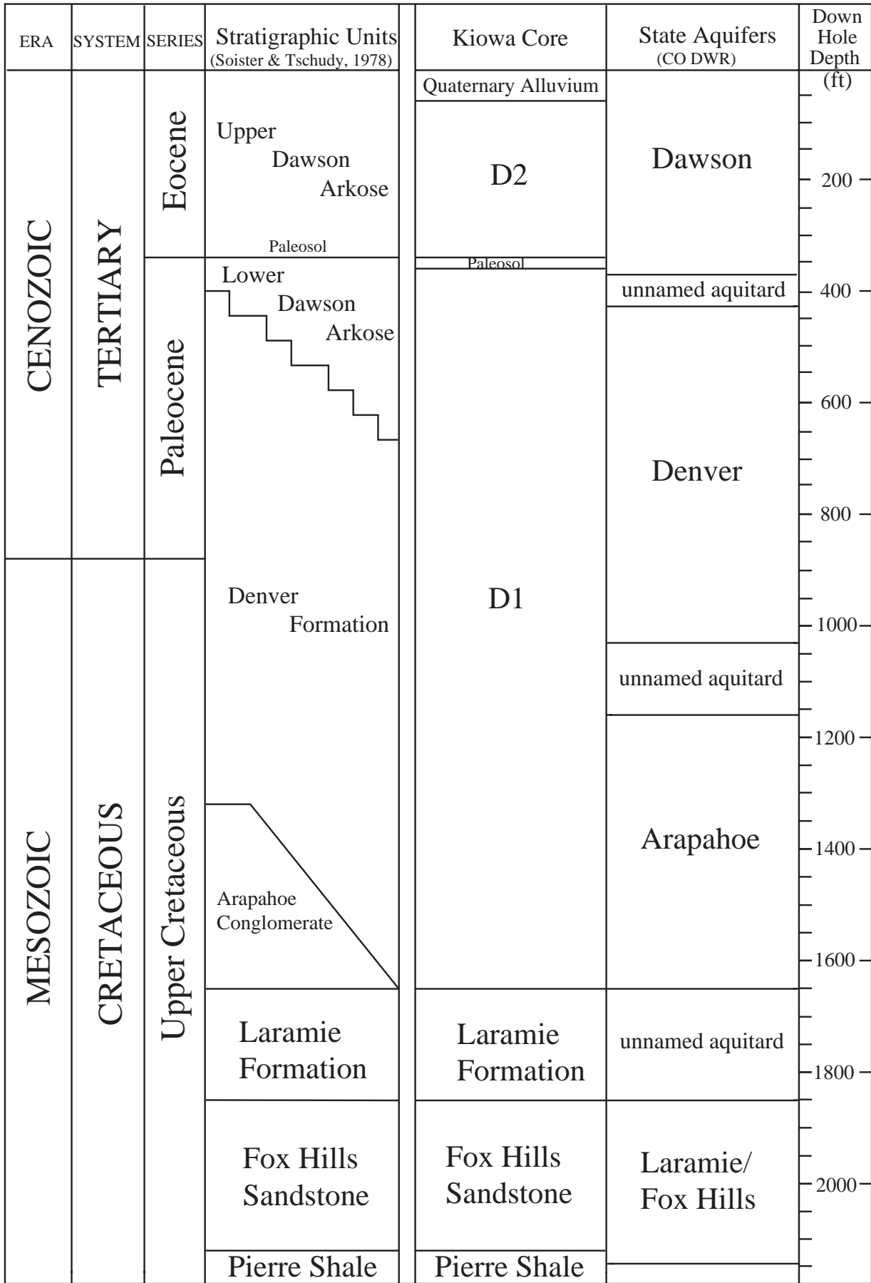
Figure 3 Chart comparing stratigraphic and hydrogeologic nomenclature in the Denver Basin, Colorado
