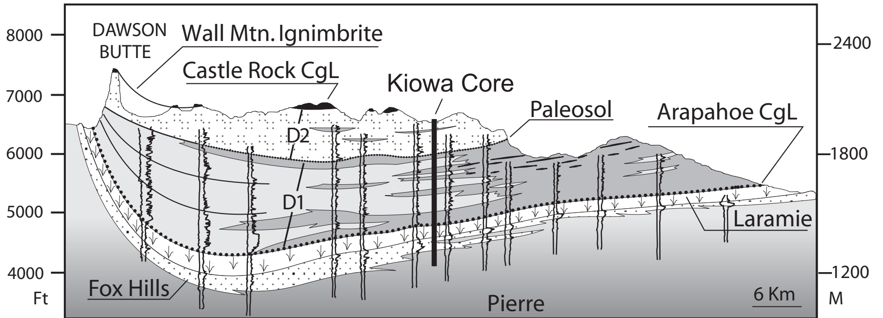
Figure 7 Generalized chart showing bedrock geology in the Denver Basin, Colorado, along cross section A-A' (location of cross section shown in figure 5)
