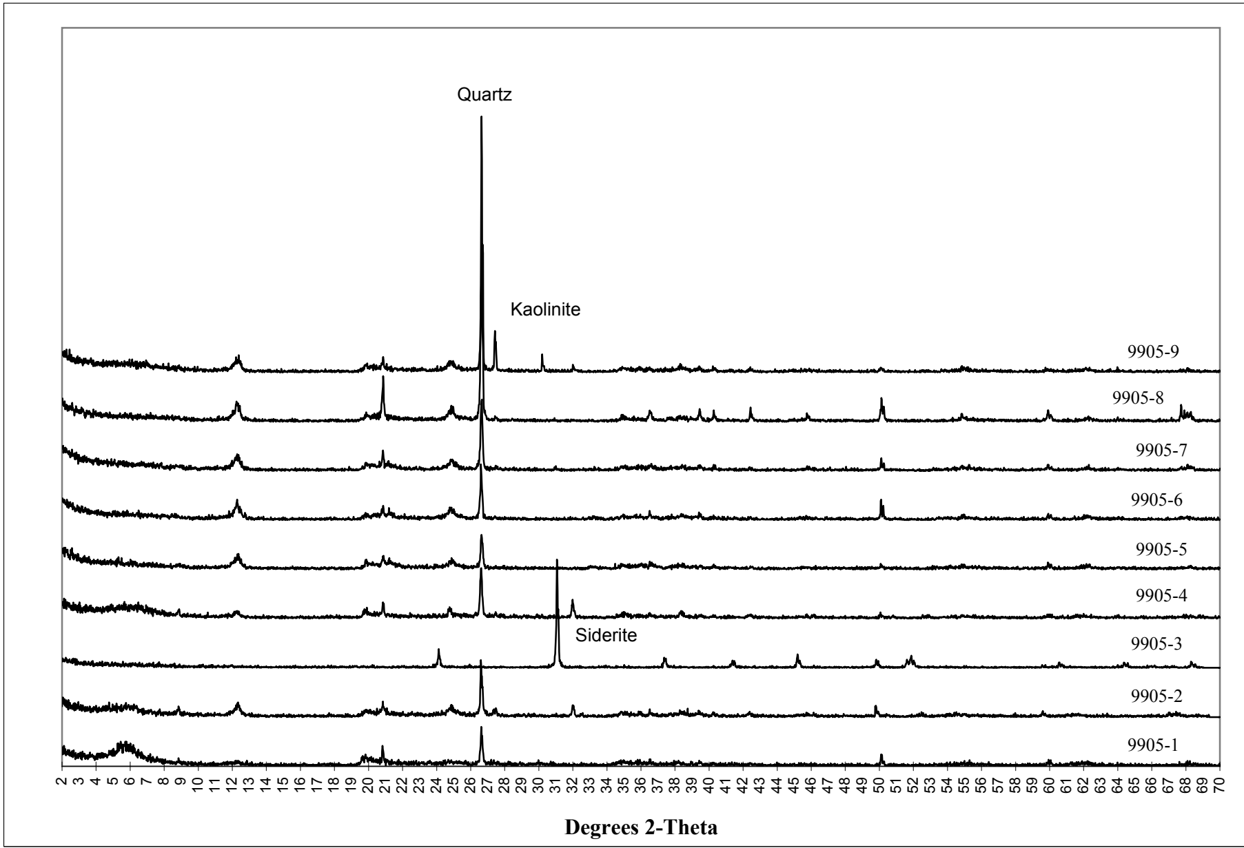
Figure 14. Paleosol Series Whole Rock XRD Patterns
