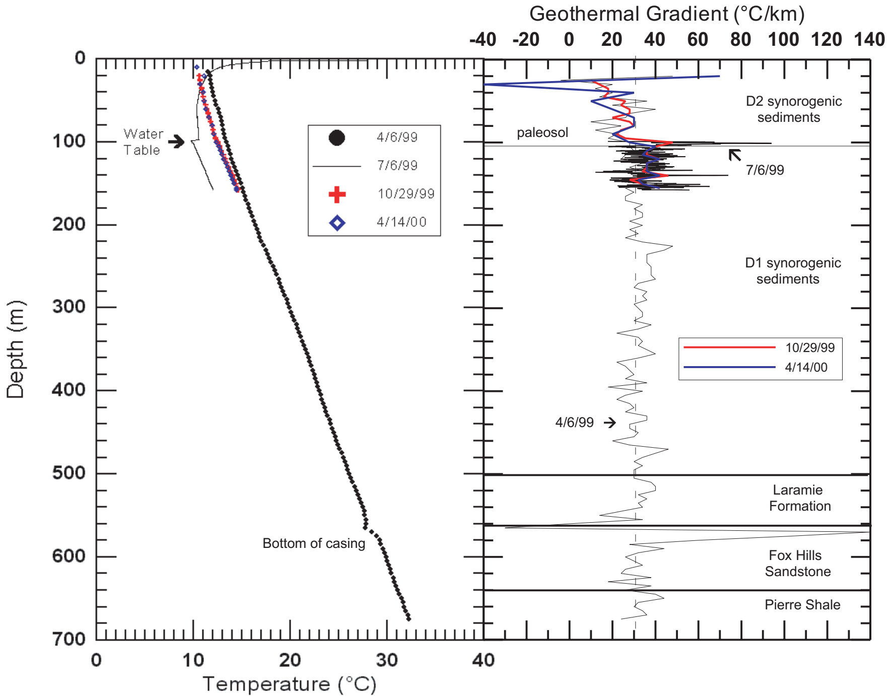
Figure 21 Temperature and gradient plots for the Kiowa #1 core
