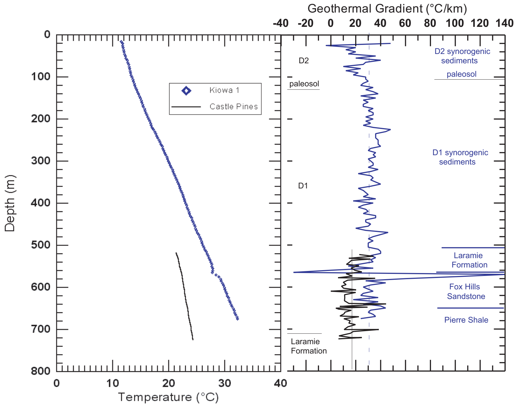
Figure 23 Comparison of temperature and gradient plots for Kiowa #1 and Castle Pines wells, Denver Basin, Colorado
