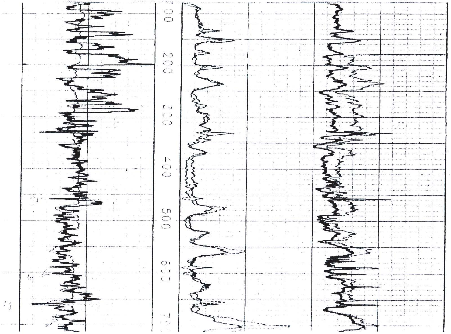
Plate 1 Electric and gamma logs from the Kiowa #1 well (page 3 of 6)
