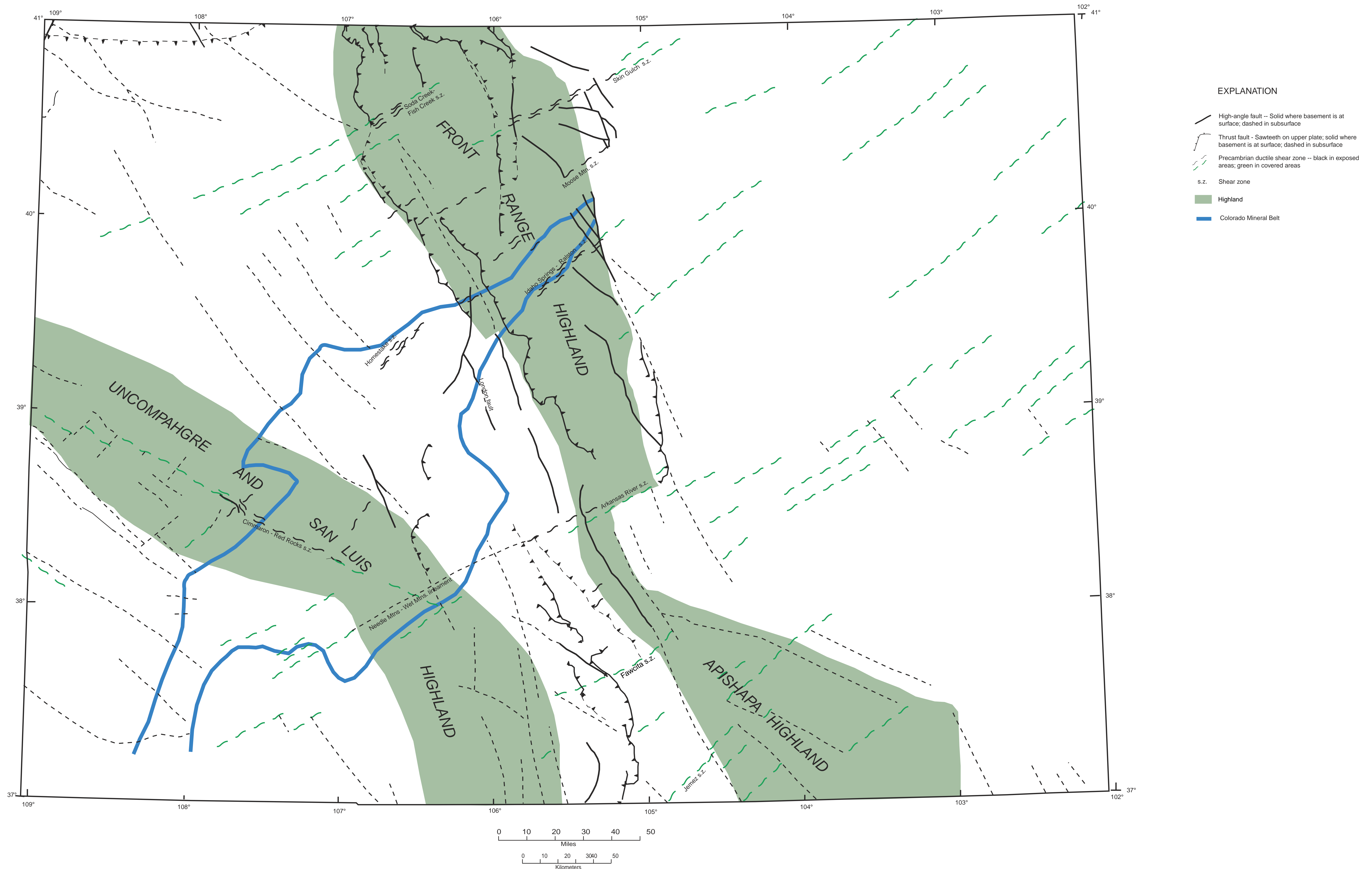
Figure 5 - Fault pattern developed during Uncompahgran disturbance of Snake River - Wichita tectonic zone
