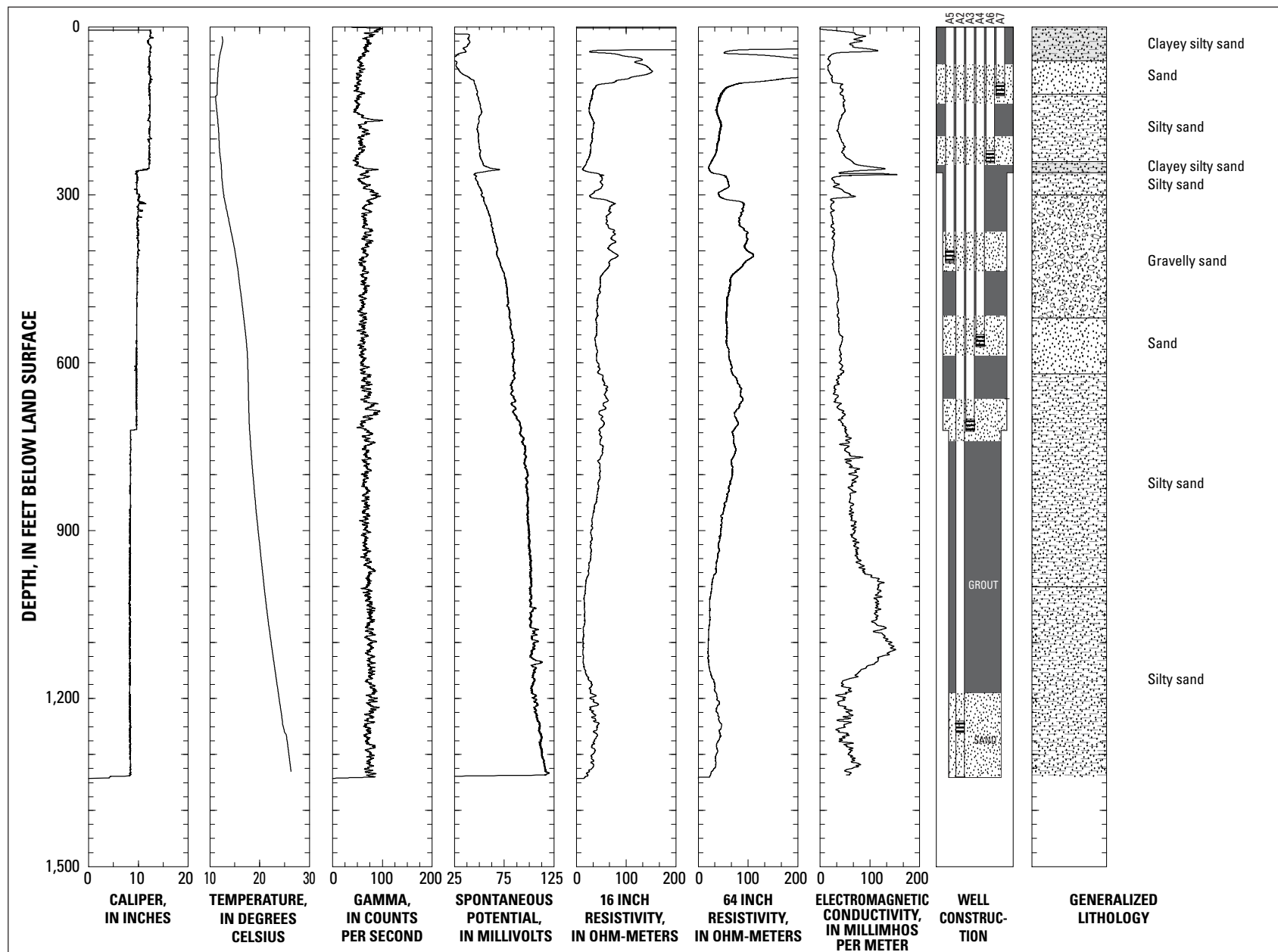
Figure 14. Geophysical logs, well-construction diagram, and generalized lithologic description for multiple-well monitoring site LOMITA-1 (4S/14W-26A2-7), Los Angeles County, California.
