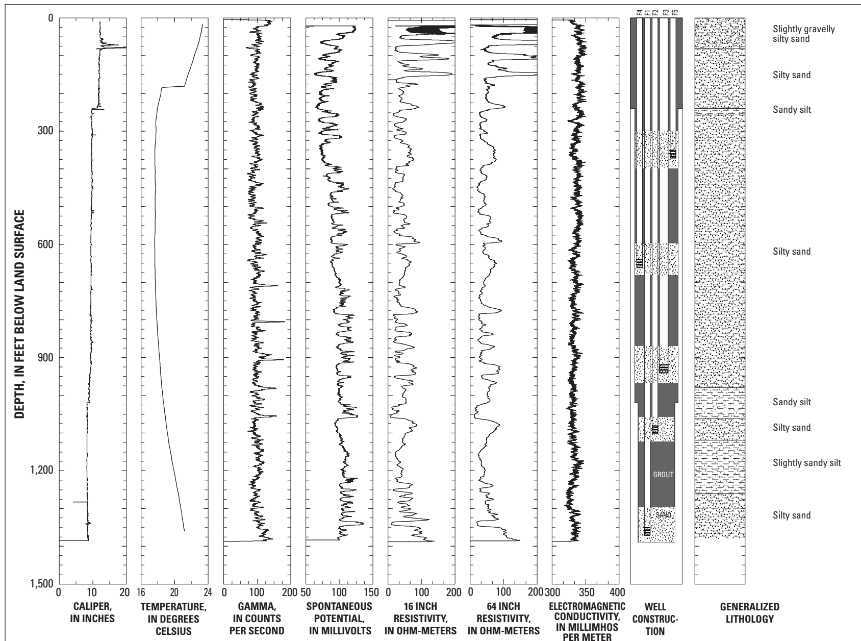
Figure 17. Geophysical logs, well-construction diagram, and generalized lithologic description for multiple-well monitoring site LOS ANGELES-1 (2S/13W-17F1-5), Los Angeles County, California.
