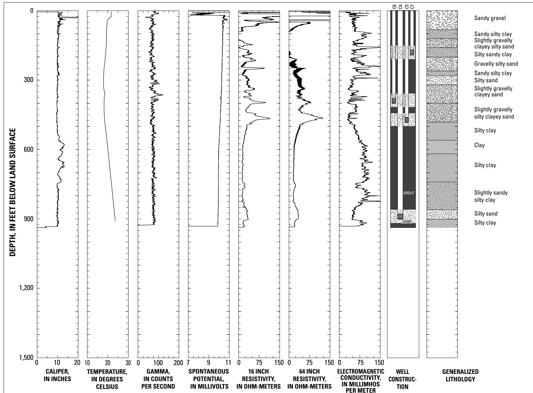
Figure 18. Geophysical logs, well-construction diagram, and generalized lithologic description for multiple-well monitoring site PICO RIVERA-1 (2S/11W-18C4-7), Los Angeles County, California.
