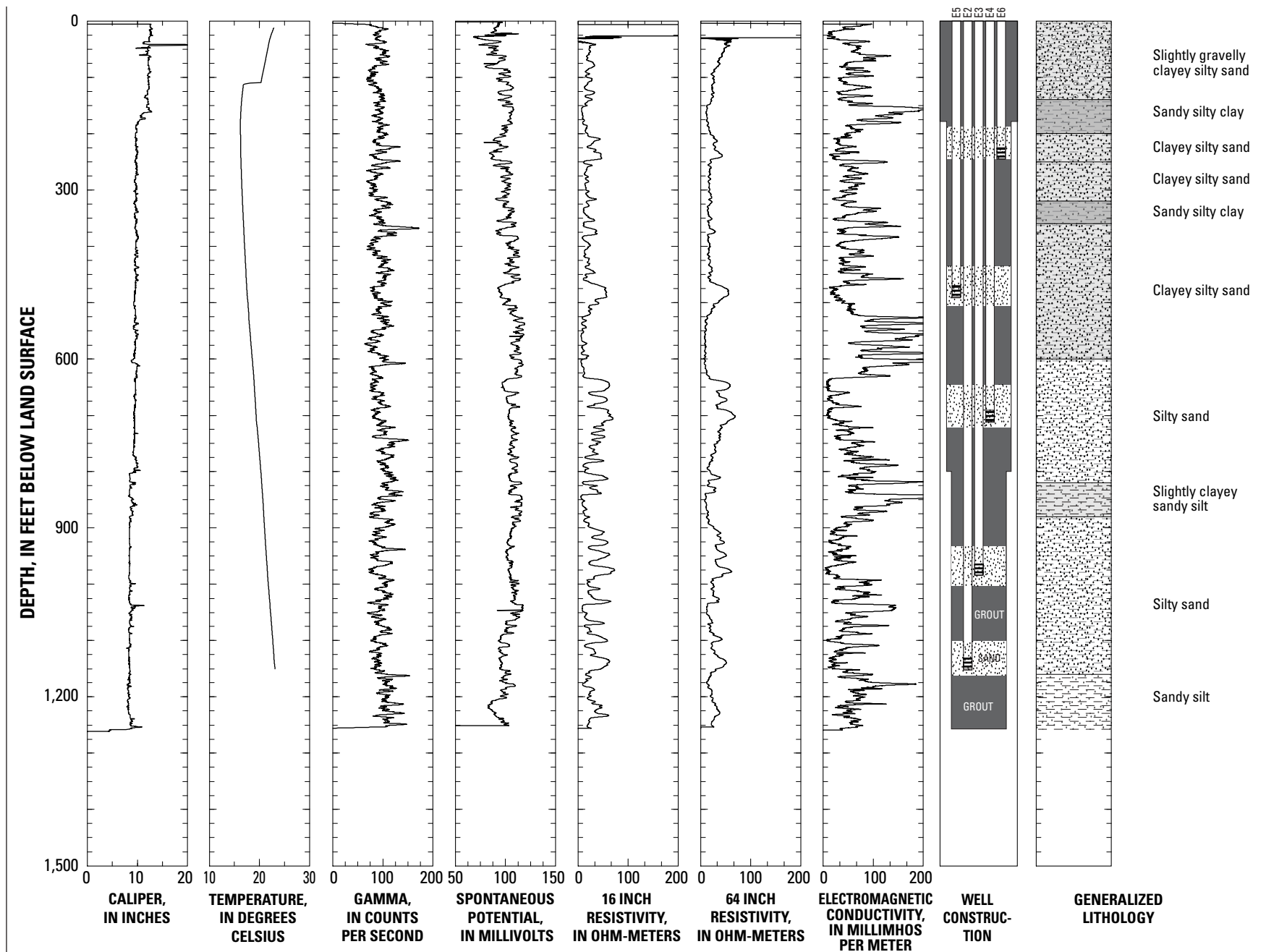
Figure 12. Geophysical logs, well-construction diagram, and generalized lithologic description for multiple-well monitoring site LA MIRADA-1 (3S/11W-26E2-6), Los Angeles County, California.
