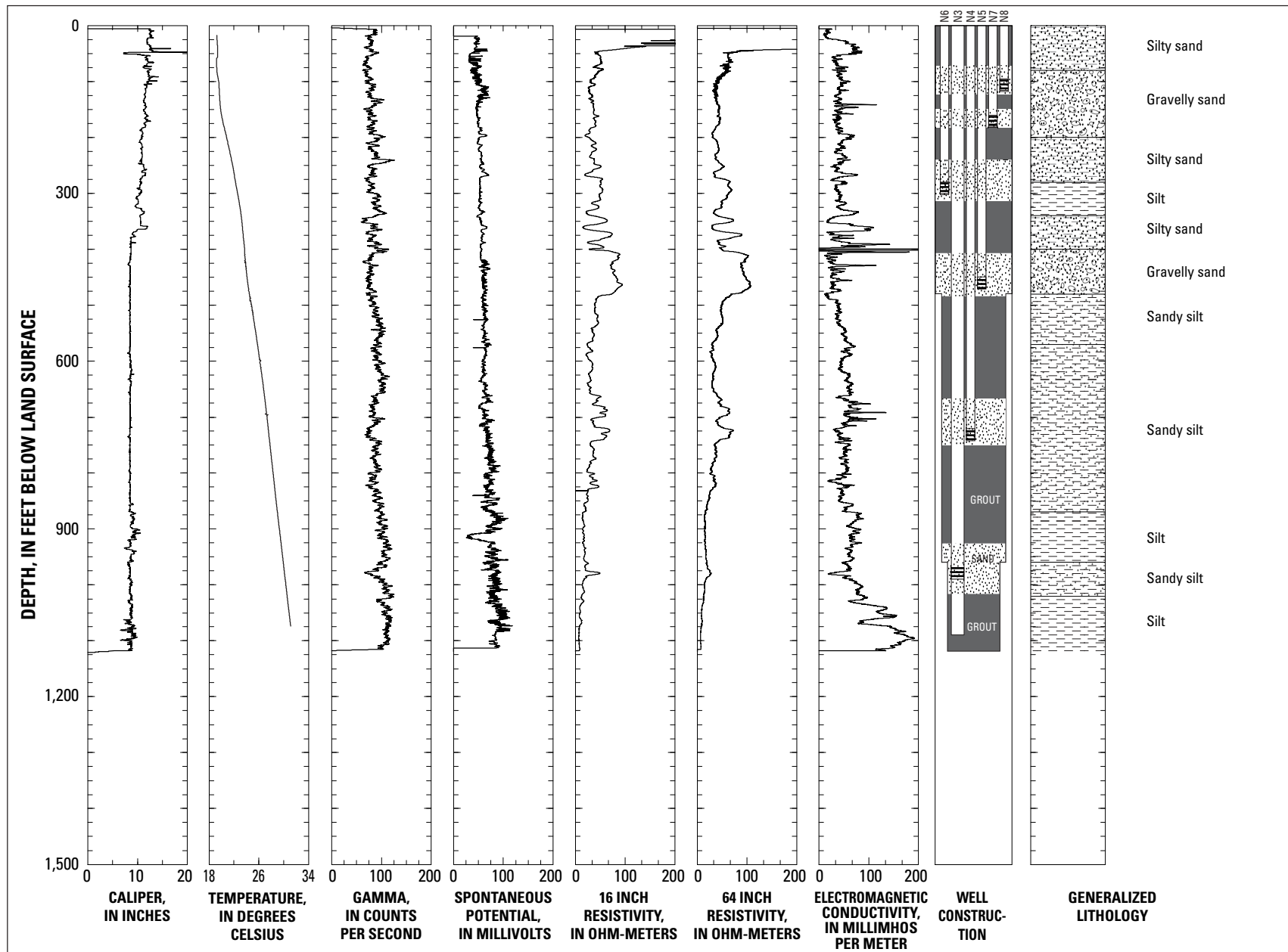
Figure 16. Geophysical logs, well-construction diagram, and generalized lithologic description for multiple-well monitoring site LONG BEACH-2 (4S/13W-1N3-8), Los Angeles County, California.
