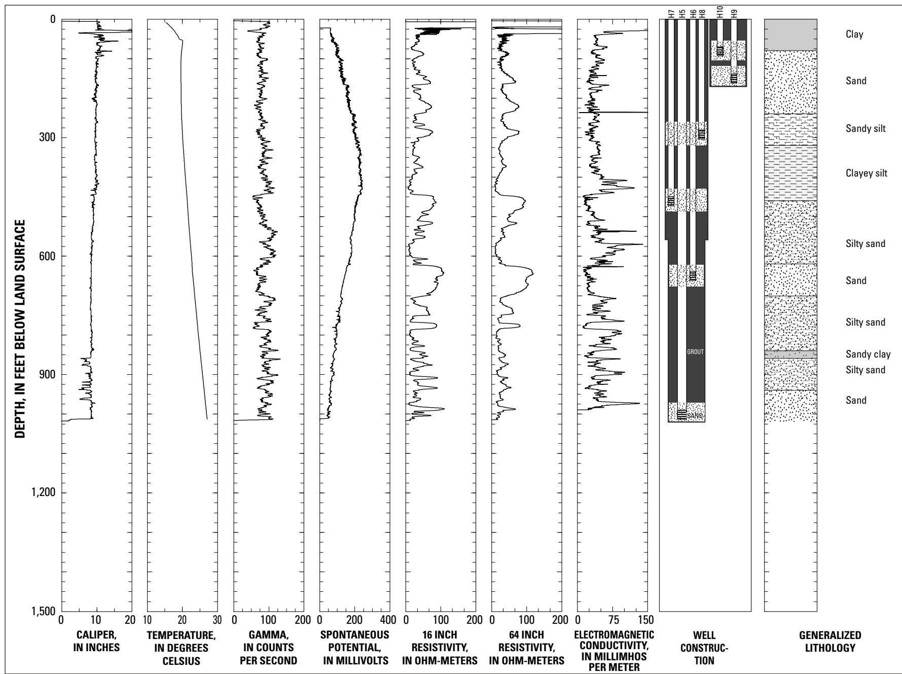
Figure 13. Geophysical logs, well-construction diagram, and generalized lithologic description for multiple-well monitoring site LAKEWOOD-1 (4S/12W-5H5-10), Los Angeles County, California.
