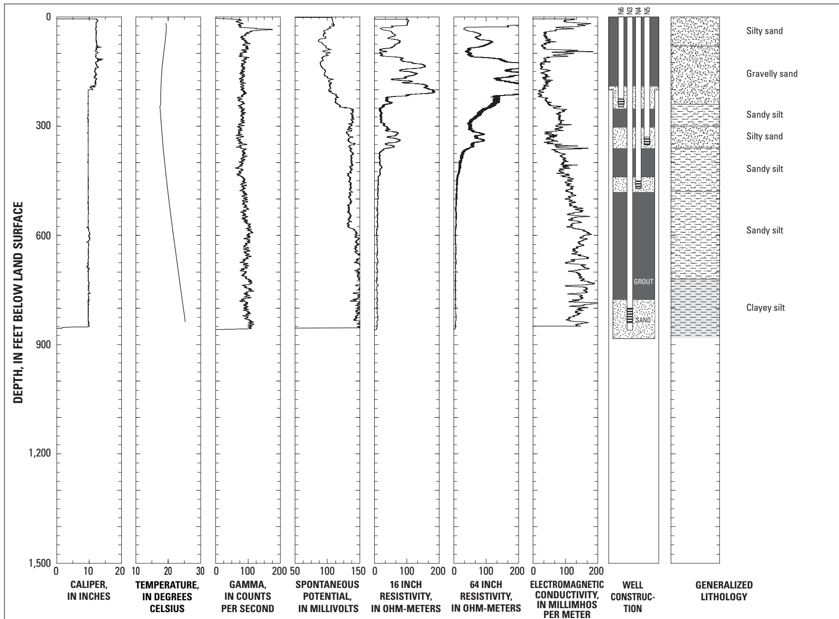
Figure 11. Geophysical logs, well-construction diagram, and generalized lithologic description for multiple-well monitoring site INGLEWOOD-2 (2S/14W-26N3-6), Los Angeles County, California.
