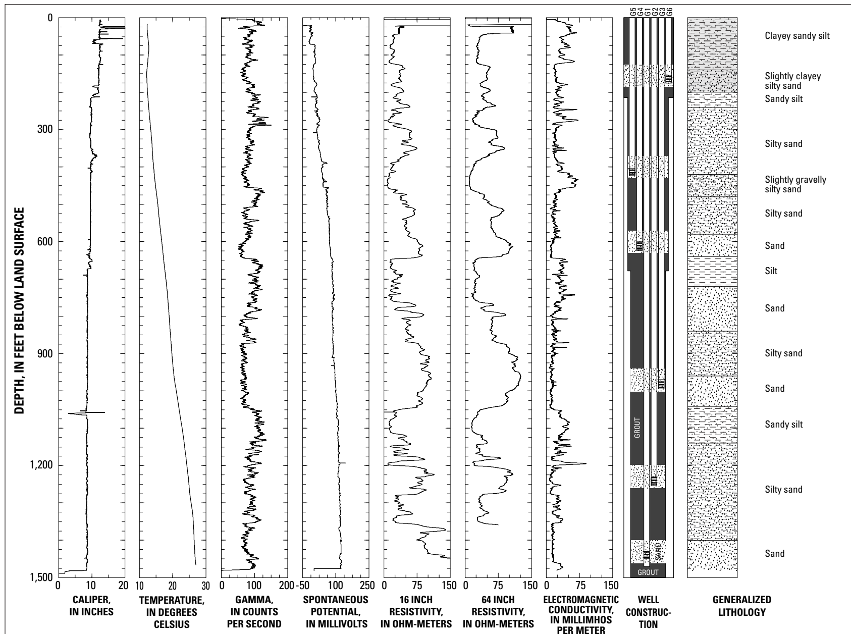
Figure 15. Geophysical logs, well-construction diagram, and generalized lithologic description for multiple-well monitoring site LONG BEACH-1 (4S/12W-25G1-6), Los Angeles County, California.
