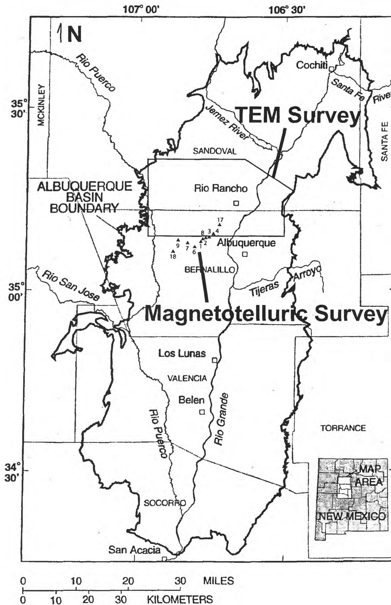
Figure 1. Index map of the Albuquerque Volcanoes survey area, west of Albuquerque, in the Middle Rio Grande basin (Albuquerque Basin Boundary), New Mexico. Solid triangles are magnetotelluric stations acquired in 1997, 1998, and 1999. TEM is outline of Rio Rancho airborne time domain electromagnetic survey. Base map modified from Bartolino (1999).
