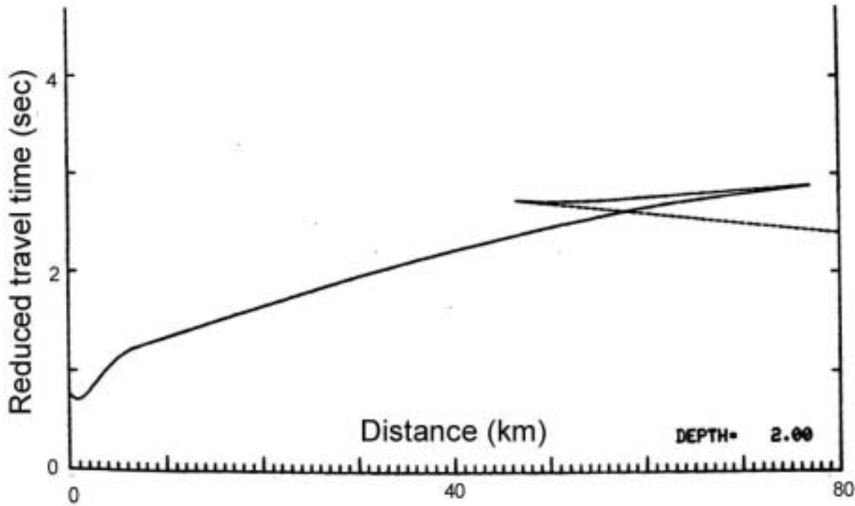
Figure 8. A sample plot of the reduced travel time curve for the above input file for a source at 2 km depth.
