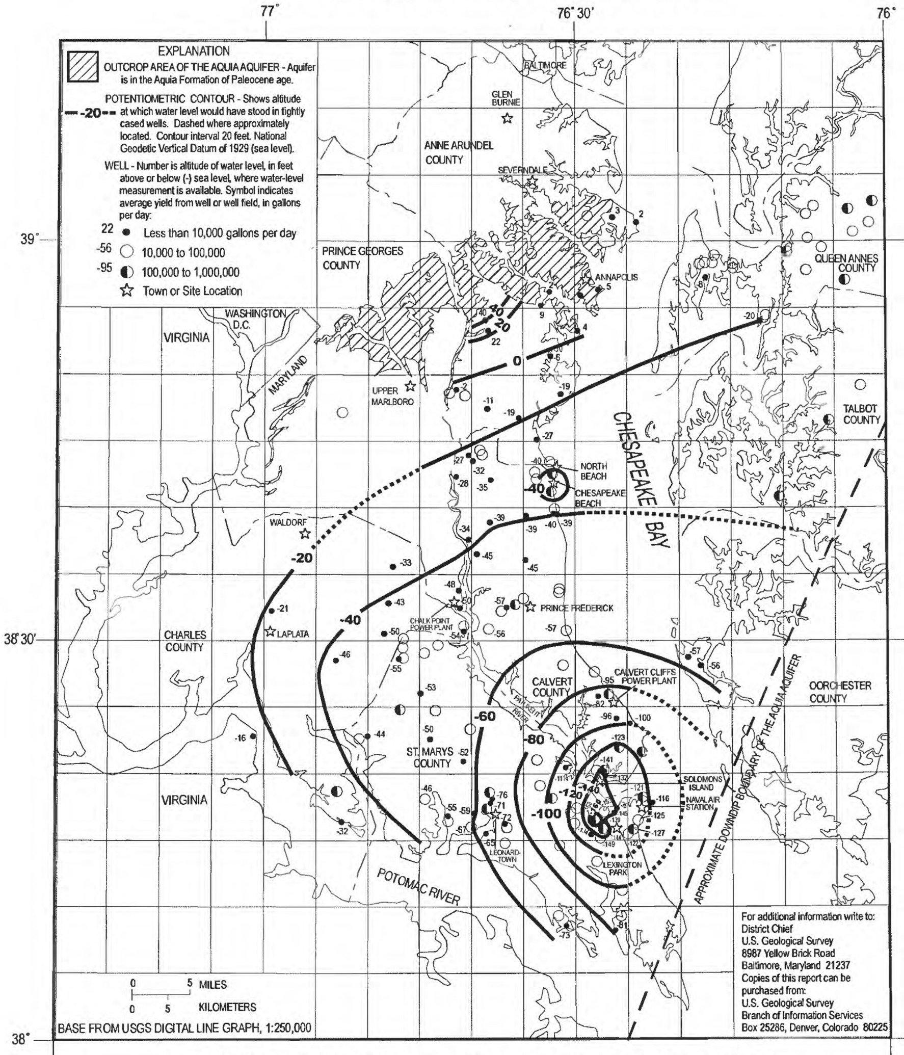
POTENTIOMETRIC SURFACE OF THE AQUIA AQUIFER IN SOUTHERN MARYLAND, SEPTEMBER 2000
