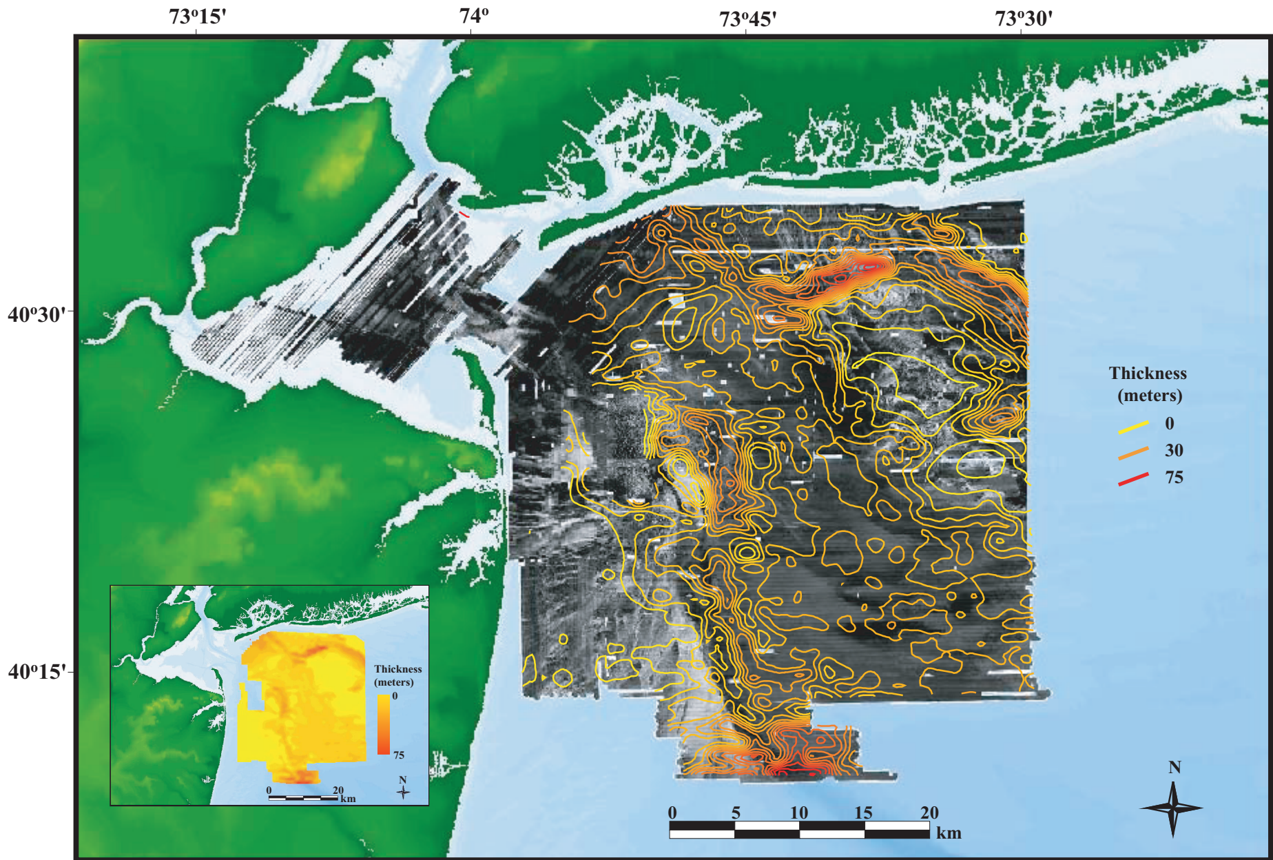
Figure 10. Isopach map showing the thickness of the Quaternary (Pleistocene and Holocene) sedimentary deposit.
