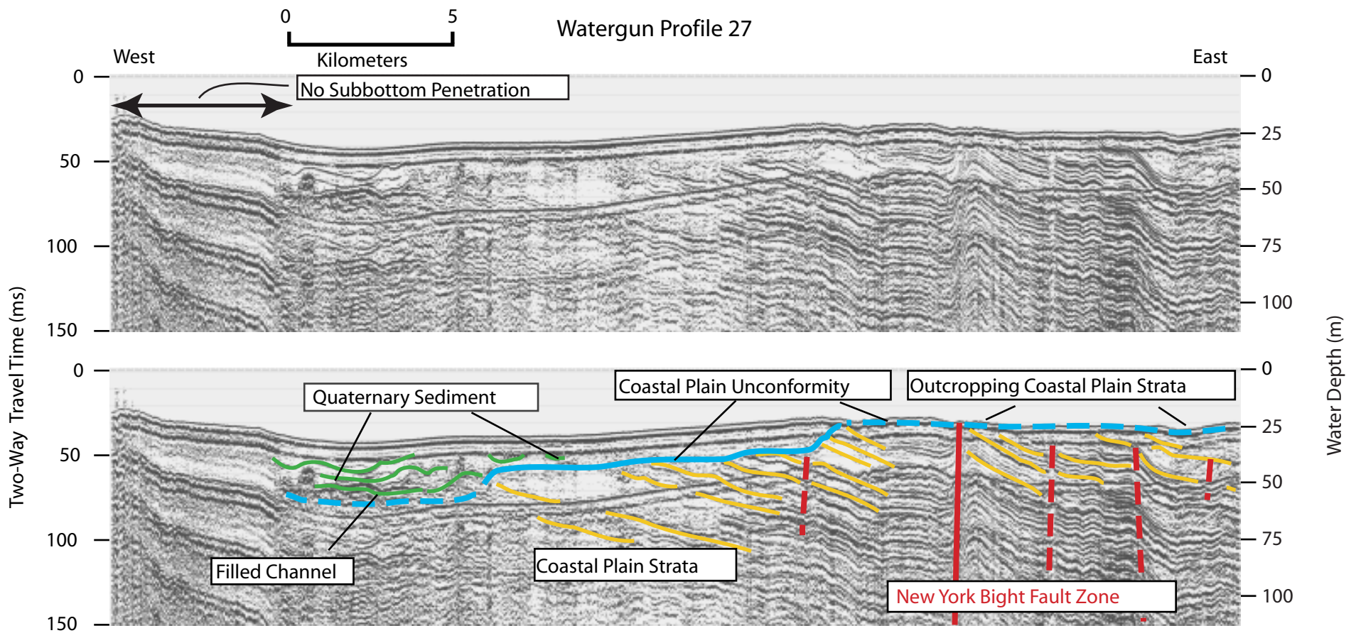
Figure 11. Representative seismic-reflection profile (cruise 95007) showing Upper Cretaceous coastal-plain strata, the overlying Quaternary sedimentary deposit, and the New York Bight fault zone. See Figure 2b for location. Water depth was calculated assuming a velocity of 1500 m/sec.
