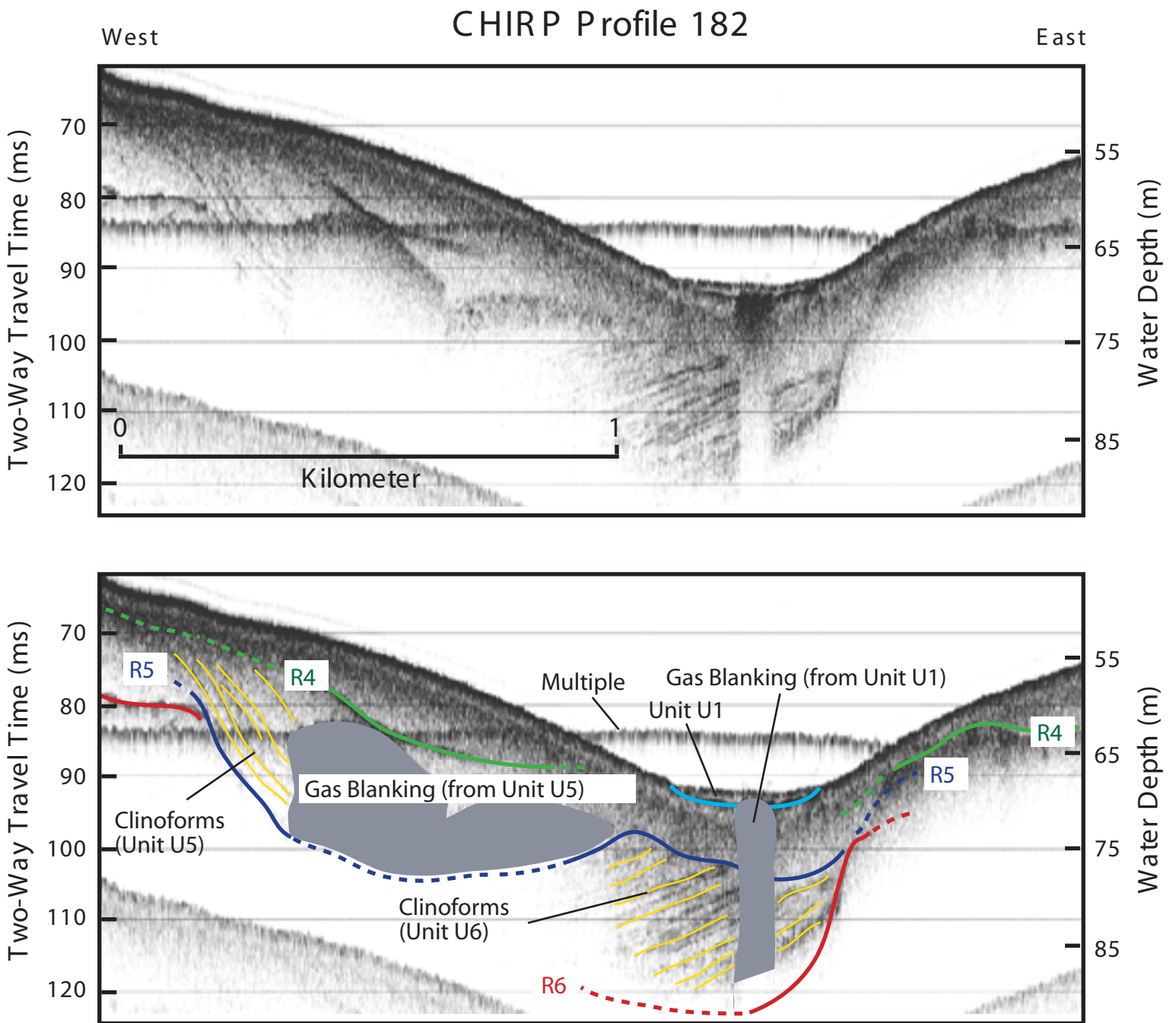
Figure 14. Representative seismic-reflection profile (cruise 96004) across the Hudson Shelf Valley showing reflector R4, Hudson channels R5 and R6, and Hudson channel-fill units U5 and U6. Gas associated with units U5 and U1 is evident as areas of acoustic blanking. See Figure 2b for location. Water depth was calculated assuming a velocity of 1500 m/sec.
