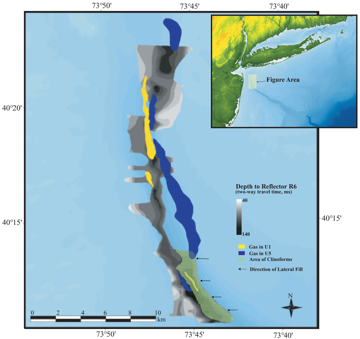
Figure 15. Map showing the depth below sea level of Hudson Channel R6 (Allison and others, 1997).
