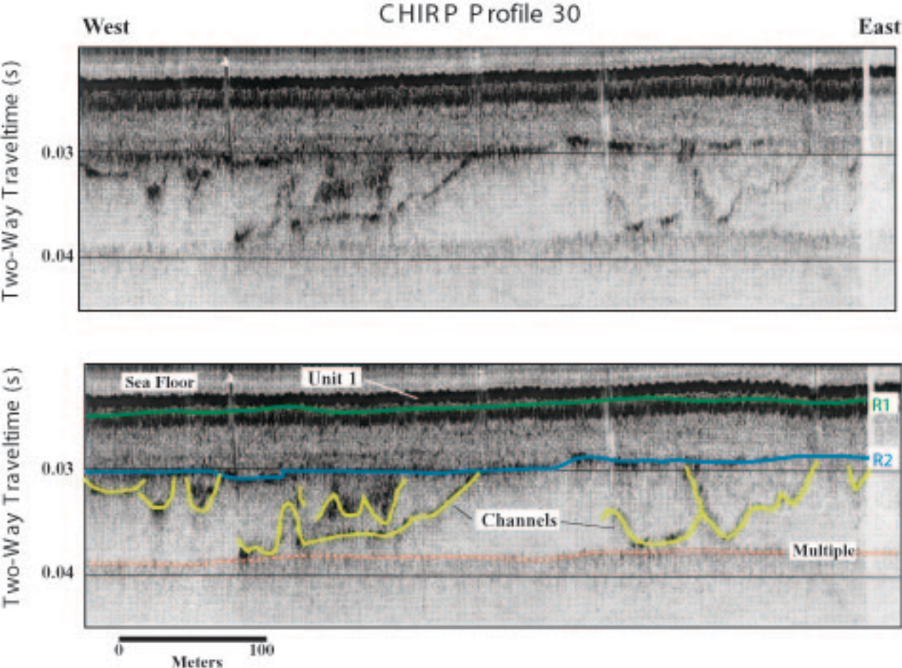
Figure 17. Representative seismic-reflection profile (cruise 95007) shows the Holocene ravinement surface (reflector R2) and an unusually strong example of reflector R1, which separates unit U1 from the underlying Holocene sedimentary deposit. The Holocene ravinement surface truncates channels which are cut into the Pleistocene sedimentary deposit. See Figure 2b for location. Profile is not corrected for towing depth of the vehicle due to failure of the pressure transducer.
