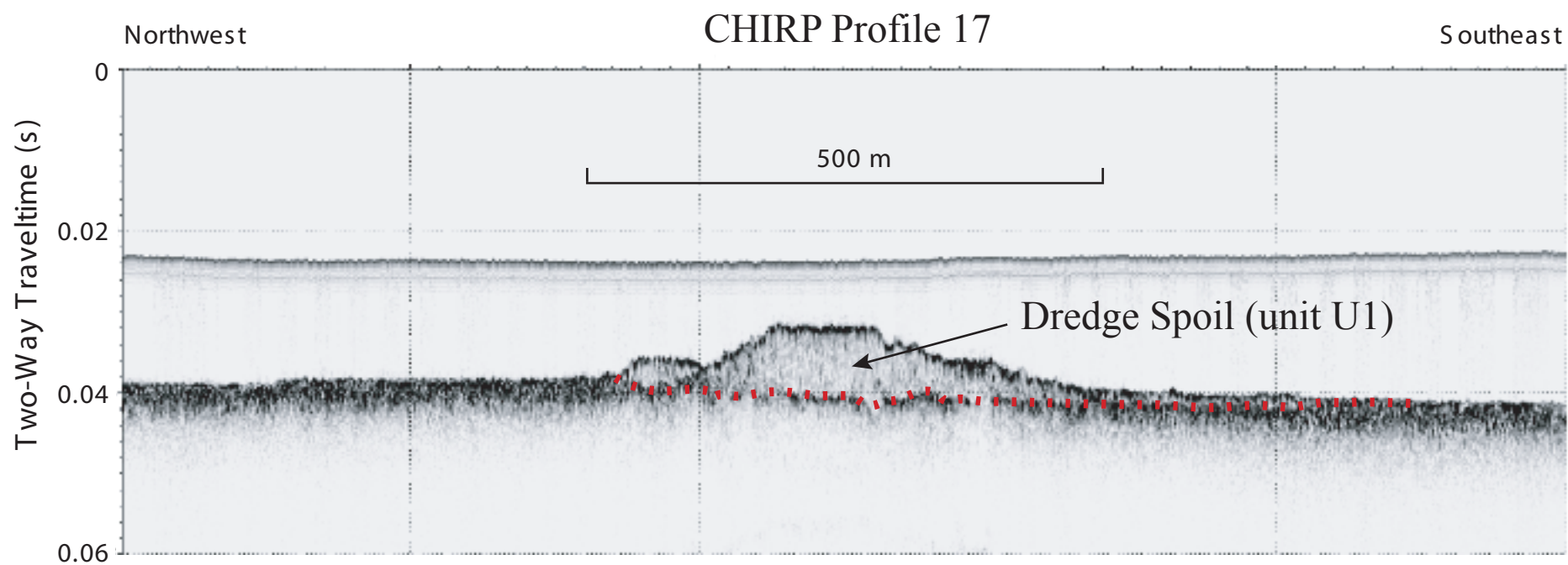
Figure 18. Seismic-reflection profile (cruise 98013) showing disposed dredged material (unit U1) in the Mud Dump Site. See Figure 2b for location.
