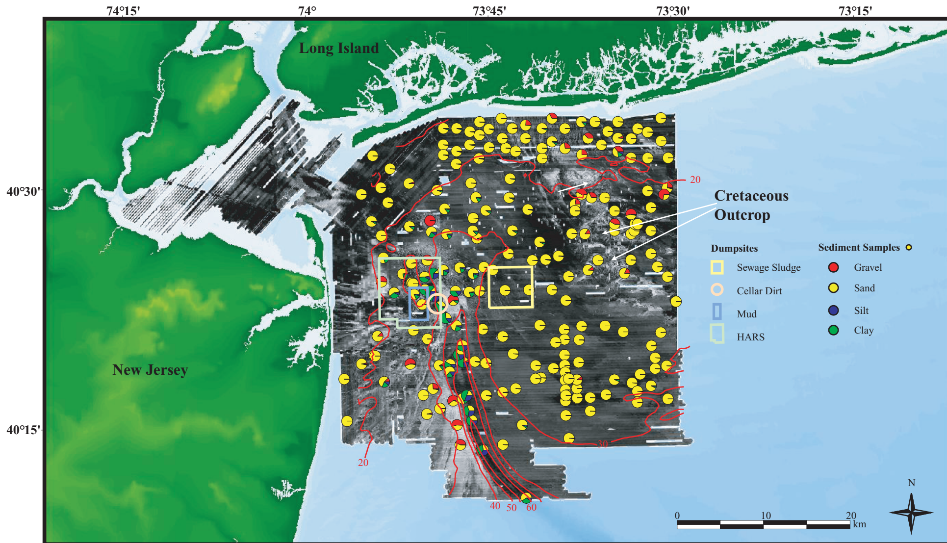
Figure 2a. Map showing sidescan-sonar imagery of the study area with overlays showing sediment sample locations, bathymetry, and dumpsite locations.
