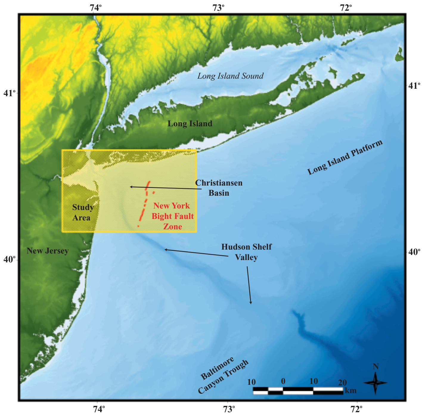
Figure 3. Index map showing the major regional geologic features of the study area.
