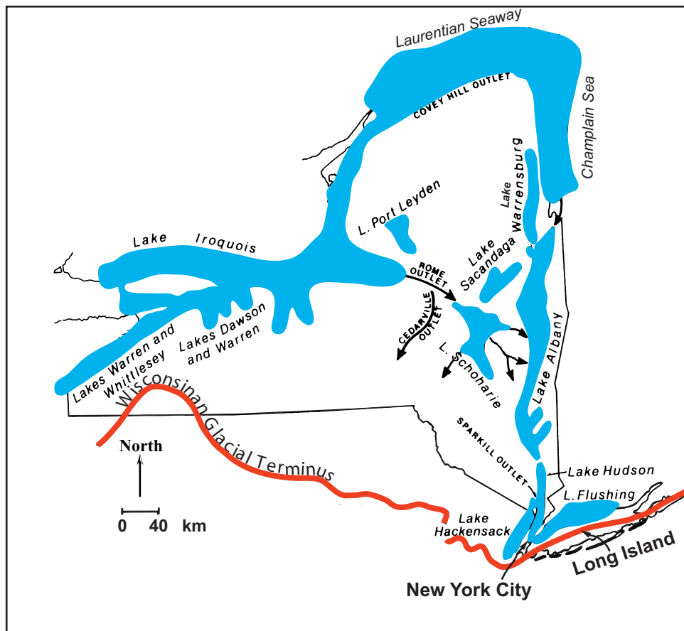
Figure 5. Map of the inferred positions of the proglacial lakes formed in the late Wisconsinan; glacial stage 2 during period of Laurentide ice sheet retreat (modified from Brigham-Grette, 1988).
